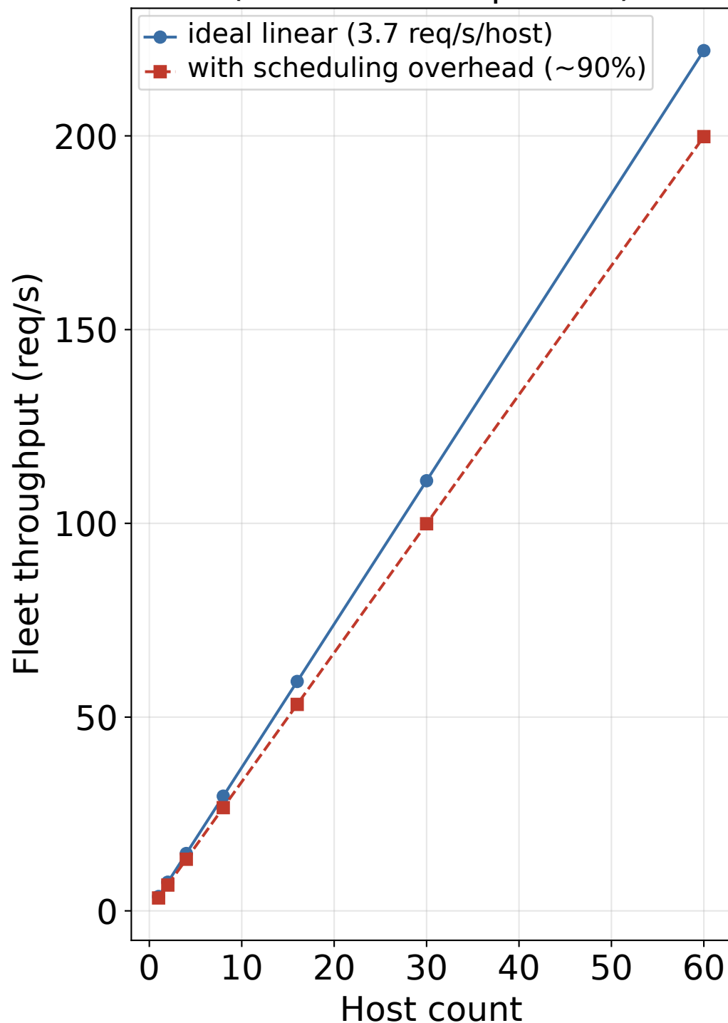
Throughput vs host count (honest 3.7 req/s/host)
