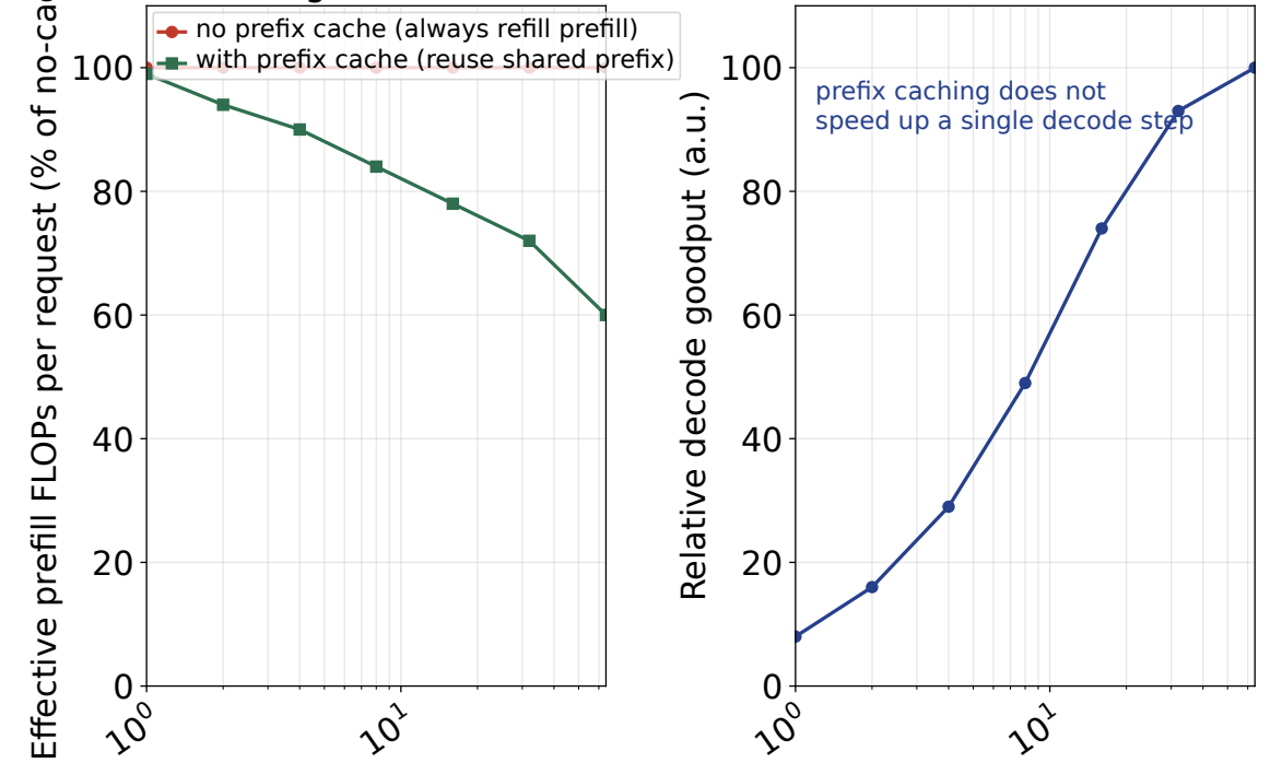
FIGURE 15.1. Decode goodput vs batch size, with and without prefix caching: caching relaxes the prefill bottleneck, not decode (illustrative, canonical decode ~25 ms/token)
