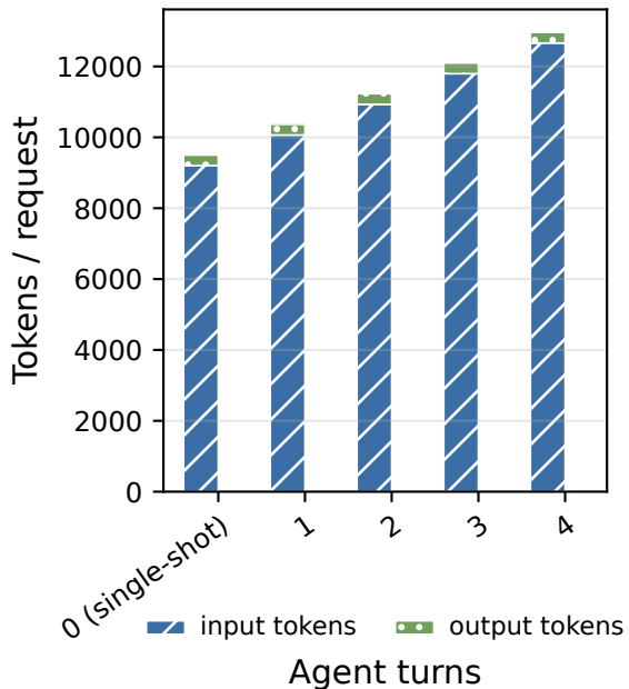
(a) Tokens accumulate
