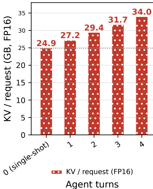
(b) KV grows 24.9 → 34.0 GB
