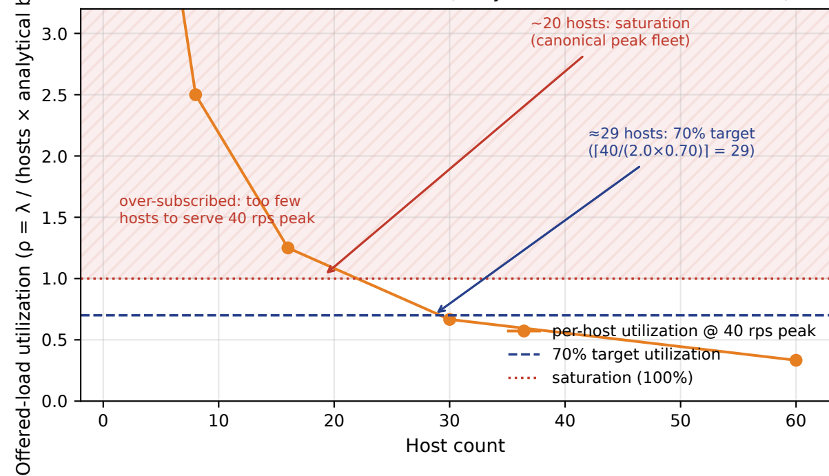
Offered-load utilization vs host count (analytical service bound, not GPU util)
