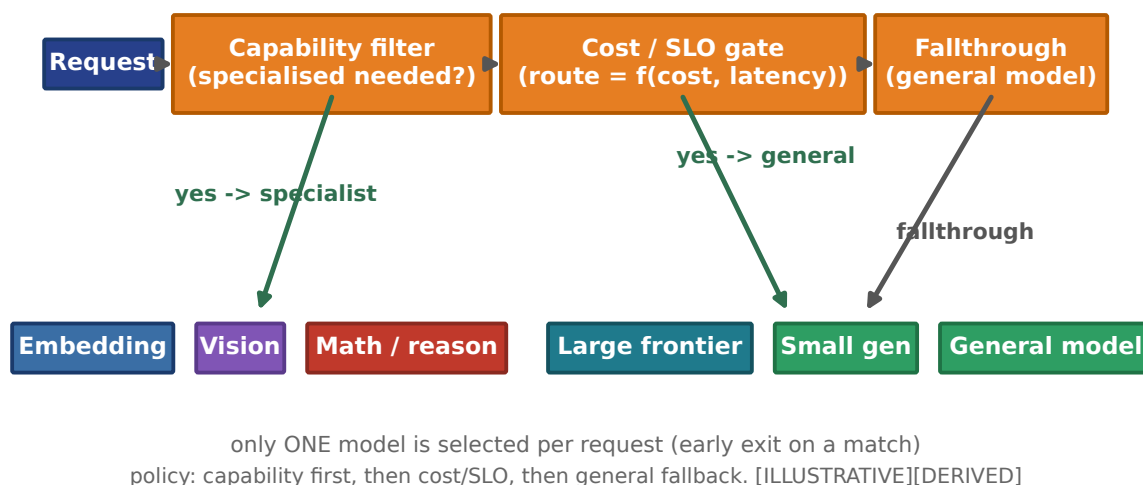
FIGURE 18.1: Model-routing decision tree: capability filter → cost/latency gate → fallback, with the five specialized families as leaves [ILLUSTRATIVE conceptual]
