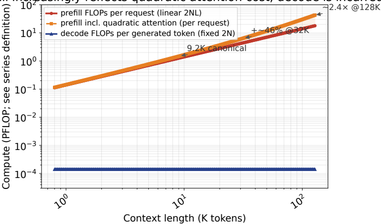
FIGURE 22.1: Full-attention prefill increasingly reflects quadratic attention cost; decode is incurred token-by-token [ILLUSTRATIVE][DERIVED]
