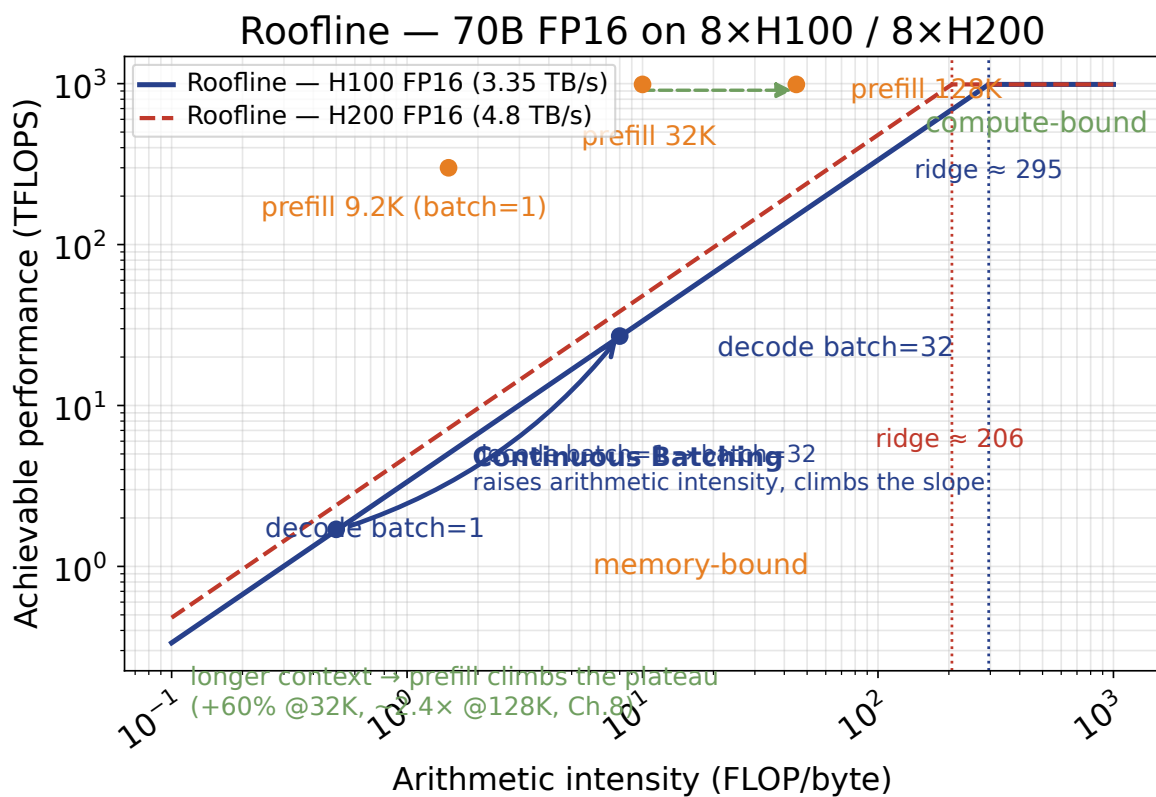
FIGURE 8.1: Prefill above the ridge (compute-bound), decode below it (memory-bound). H100 (solid) vs H200 (dashed) ridge points from vendor datasheets (989 TFLOPS dense, 3.35 / 4.8 TB/s); Continuous-Batching arrow shows decode climbing the slope as batch grows [DERIVED from 1P: vendor datasheet]
