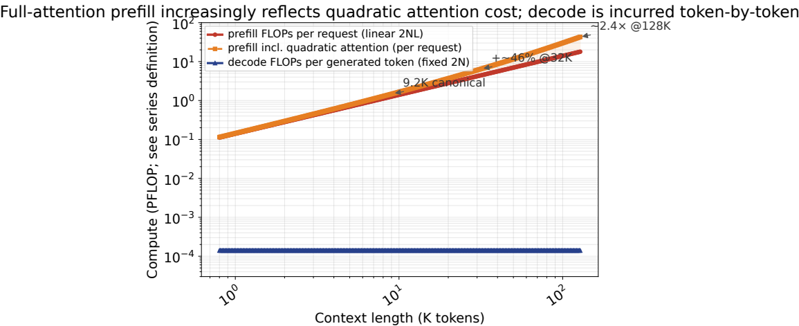
FIGURE 22.1: Full-attention prefill increasingly reflects quadratic attention cost; decode is incurred token-by-token [2° DERIVED]
