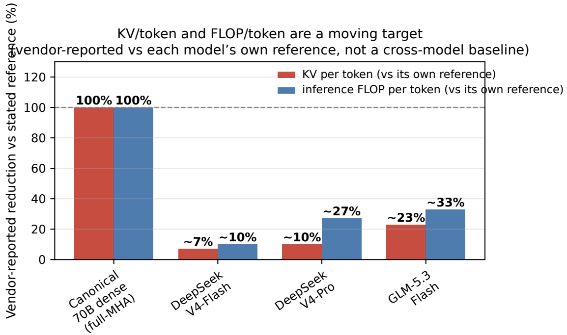
FIGURE A.2: The KV constant and FLOP/token are a moving target: hybrid attention cuts both at the mechanism. A canonical 70B dense full-MHA is shown at 100% for scale; the frontier percentages are each model's vendor-reported reduction versus its own stated reference (e.g. DeepSeek V4 vs V3.2), not a cross-model percentage of the canonical 70B [DERIVED from 1P claims: arXiv 2606.19348; HF zai-org]
