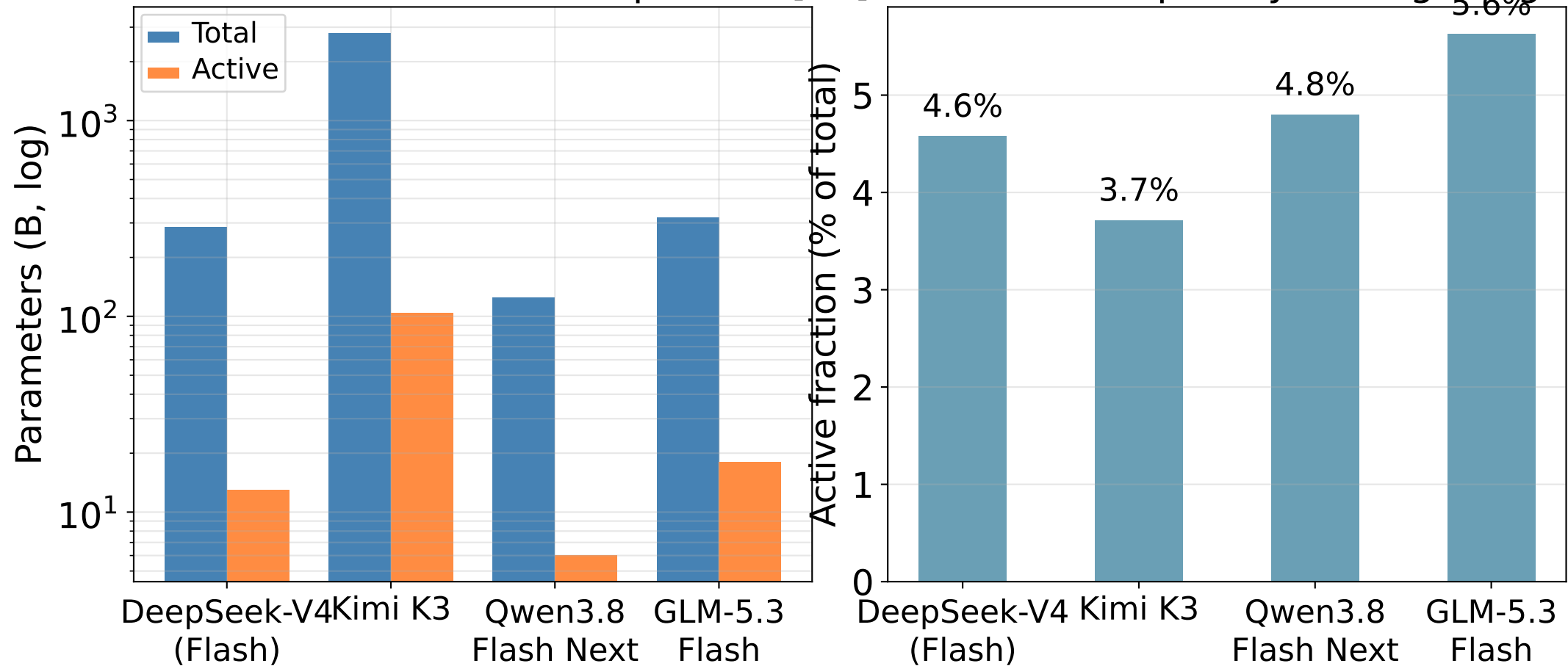
Frontier MoE: total vs active params [1P]Extreme MoE sparsity — single digits
