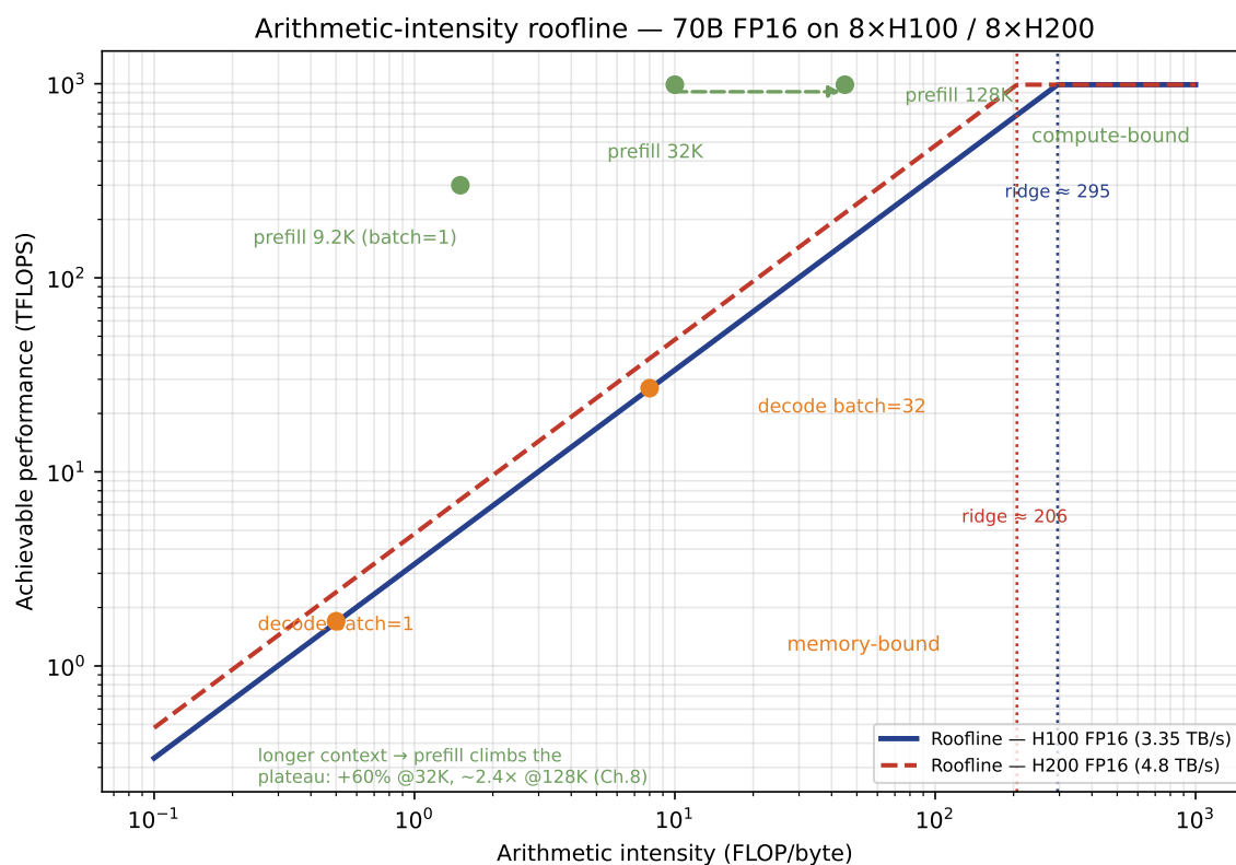
FIGURE 8.1. Fig 8.1 — Prefill above the ridge (compute-bound), decode below it (memory-bound) [2° DERIVED]
