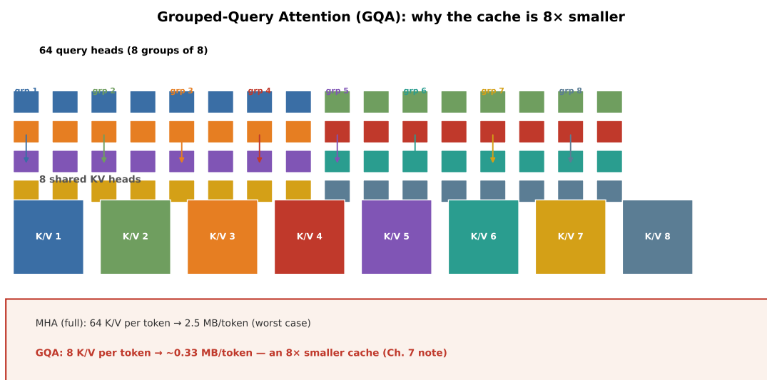
FIGURE 7.1. Fig 7.3 — Grouped-Query Attention: 64 query heads share 8 KV heads, cutting per-token KV 8× from 2.5 MB to ~0.33 MB (ILLUSTRATIVE, after LLaMA-2 70B head layout)
