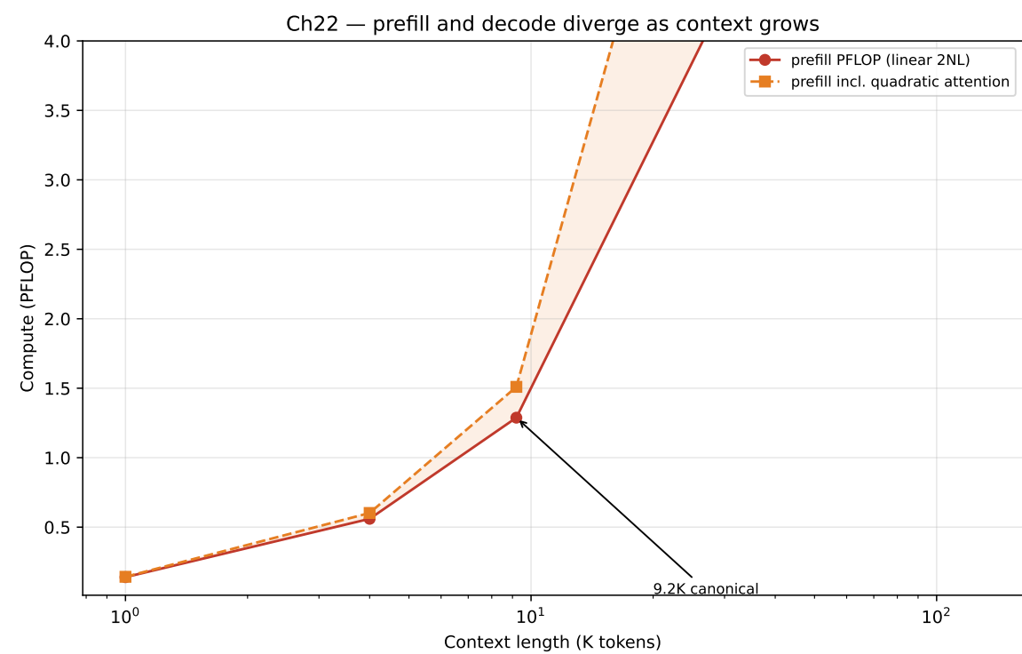
FIGURE 22.1. Fig 22.1 - Prefill vs decode bottleneck divergence [2° DERIVED]
