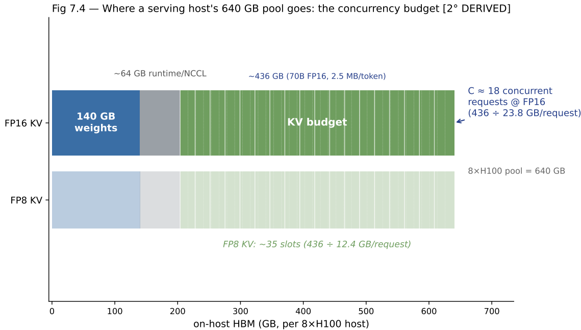
FIGURE 7.4. Fig 7.4 — The concurrency budget: where a 70B host's 640 GB pool goes [2° DERIVED]
