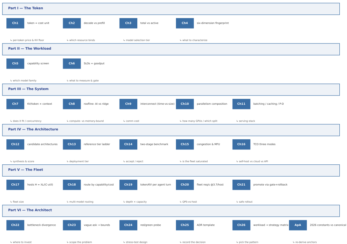
FIGURE 2. Reading the book by number. Each chapter supplies a derived quantity — a token/KV floor, a roofline point, a fleet size — and that quantity feeds a decision. Reading down a Part’s strip gives the layer-by-layer thread; reading across any chapter’s chip shows which number to reach for to answer a given question. [ILLUSTRATIVE]
