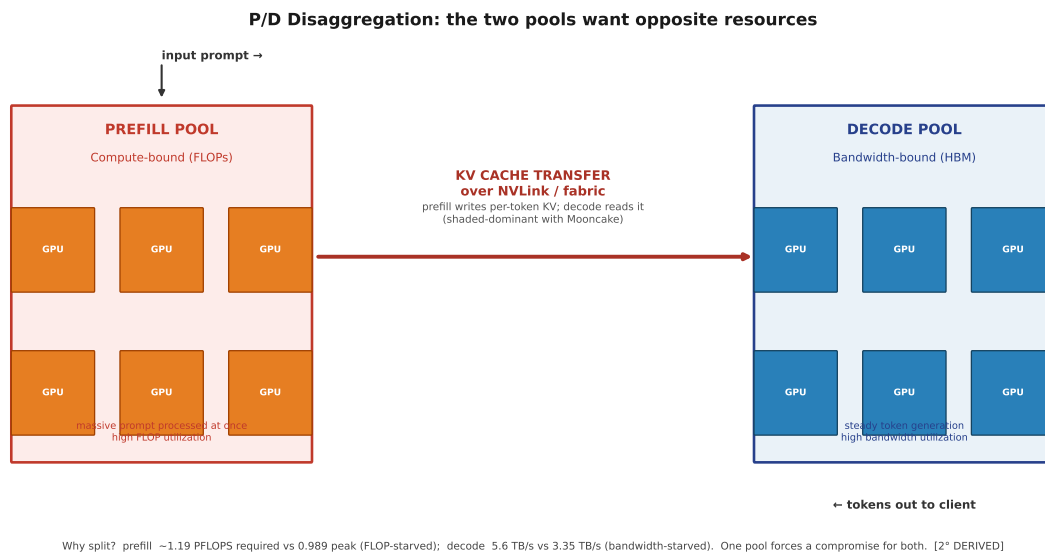
FIGURE 11.3. Fig 11.3 — P/D disaggregation topology: prefill pool (compute-bound) and decode pool (bandwidth-bound) bridged by KV transfer [2° DERIVED]
