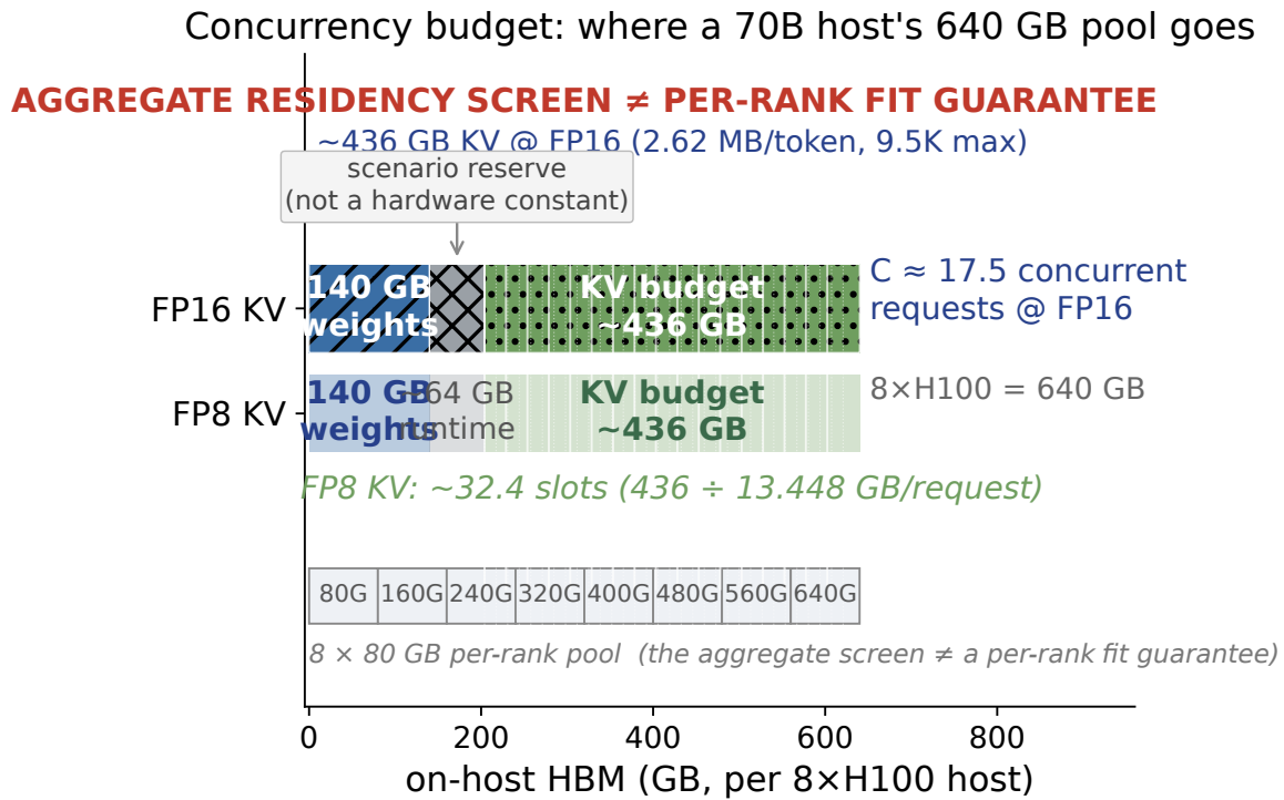
FIGURE 7.4: The concurrency budget: where a 70B host's 640 GB pool goes. Aggregate-feasibility caveat: the 640 GB figure is an aggregate across eight 80-GB H100s, not a single freely-allotable heap. Whether a given allocation actually fits depends on tensor-parallel sharding, KV partitioning, replication, runtime layout, per-rank fragmentation, workspace requirements, and communication topology — so “total bytes < total HBM” is a necessary but not sufficient test. Per-rank fit and sharding must also be validated (Chapters 9–10). [ILLUSTRATIVE][DERIVED]
