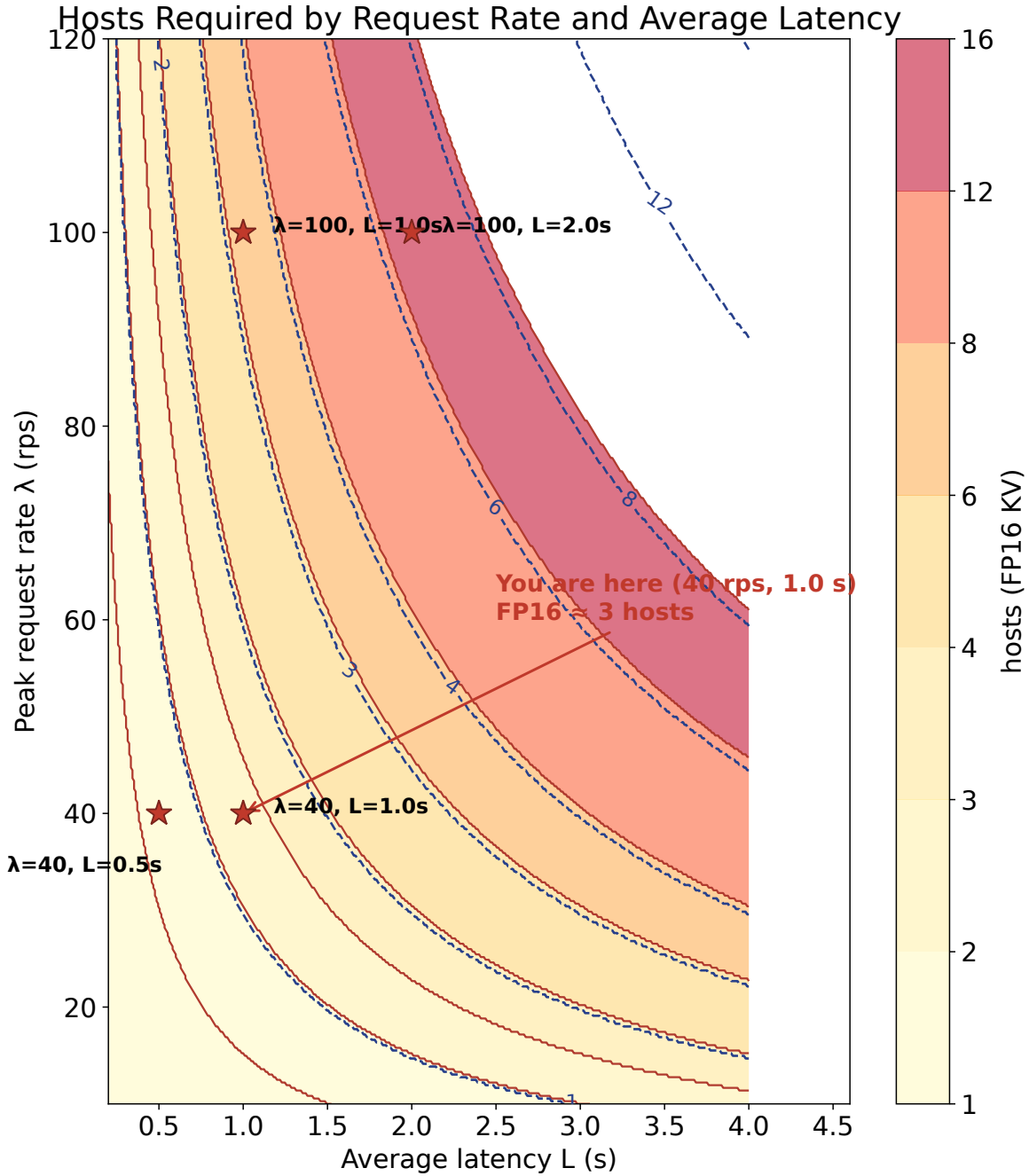
FIGURE 17.2: Hosts required by request rate and average latency, with the FP16-KV family ( C \approx 18 , filled) and the FP8-KV family ( C \approx 35 , dashed). Each contour is a fixed integer host count, H = \text{ceil}(\lambda_{\text{peak}} * L / (C * \text{util})) [DERIVED: Ch17 §3 + Ch7 KV constants]
