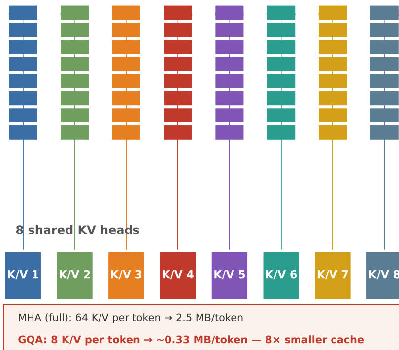
FIGURE 7.1. Grouped-Query Attention: 64 query heads share 8 KV heads, cutting per-token KV 8× from 2.5 MB to ~0.33 MB (illustrative, after LLaMA-2 70B head layout)
