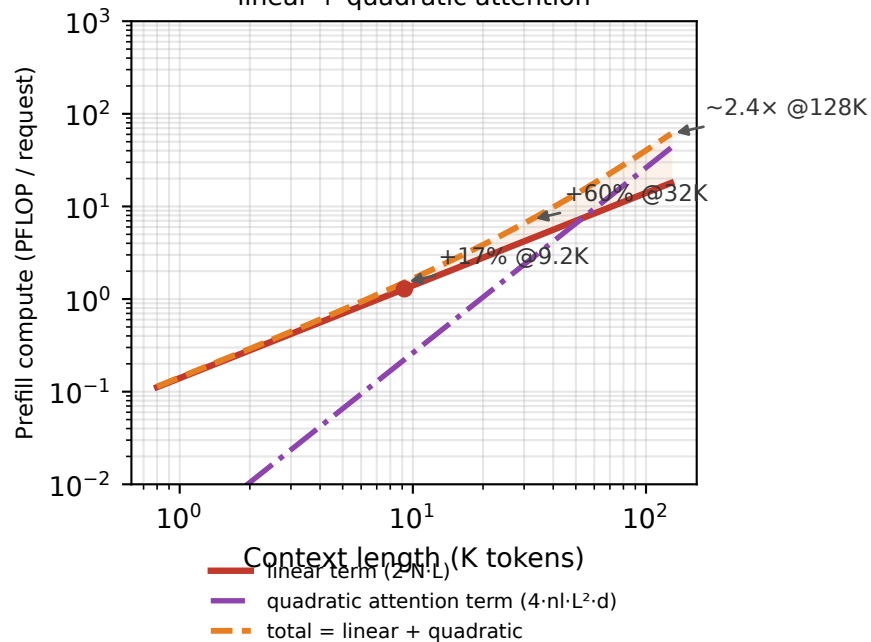
Prefill per request (decomposed): linear + quadratic attention
