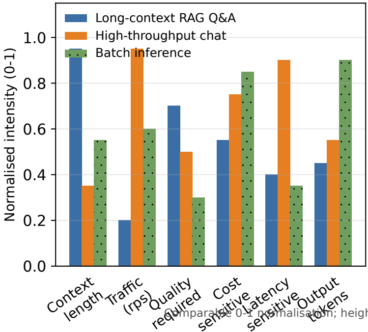
Workload fingerprints on six comparable axes (grouped bars, not radar)
