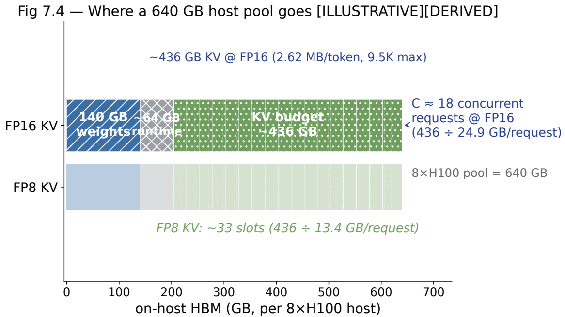
FIGURE 7.4: The concurrency budget: where a 70B host’s 640 GB pool goes. Aggregate-feasibility caveat: the 640 GB figure is an aggregate across eight 80-GB H100s, not a single freely-allotable heap. Whether a given allocation actually fits depends on tensor-parallel sharding, KV partitioning, replication, runtime layout, per-rank fragmentation, workspace requirements, and communication topology — so “total bytes < total HBM” is a necessary but not sufficient test. Per-rank fit and sharding must also be validated (Chapters 9–10). [ILLUSTRATIVE][DERIVED]
