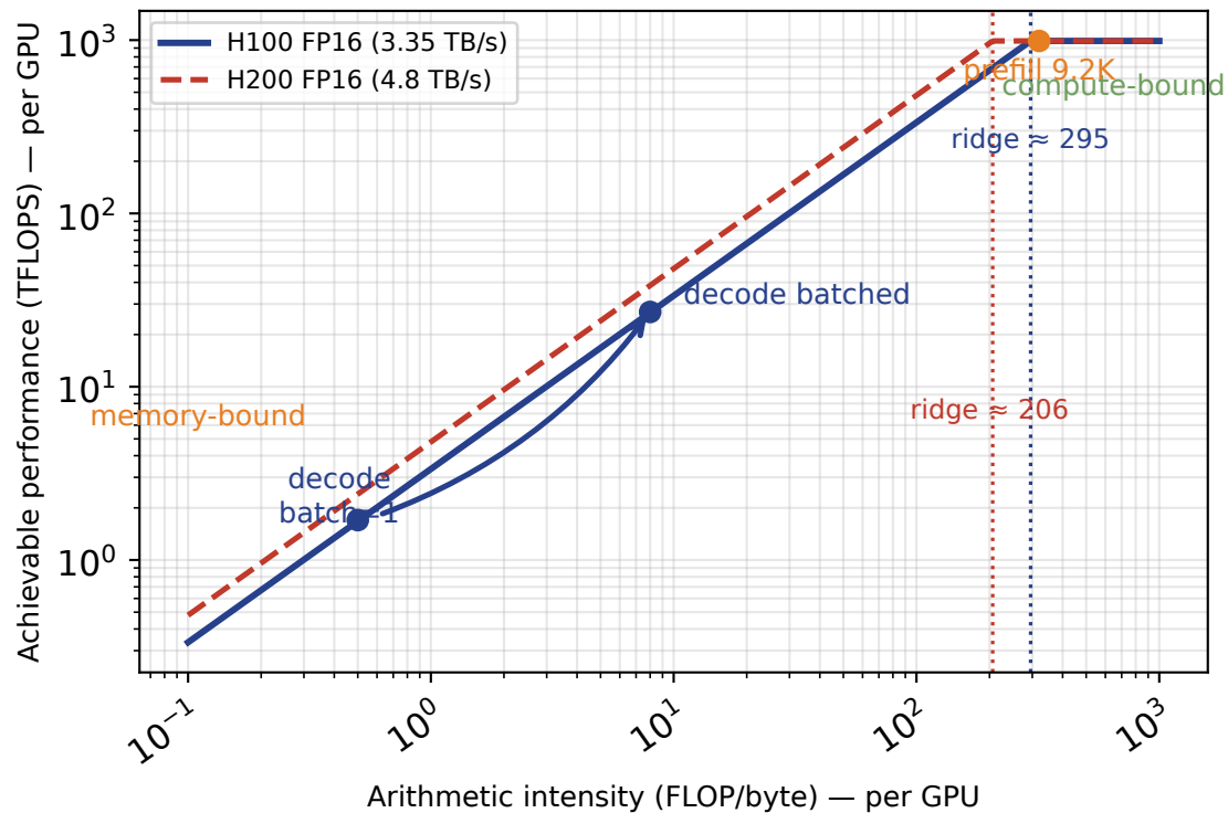
Per-GPU roofline: dense FP16, one H100 vs one H200
