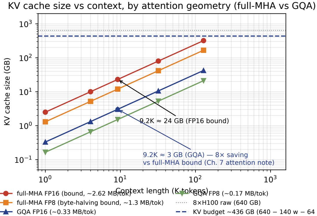
FIGURE 7.2: KV cache size vs context length for the canonical 80-layer reference geometry: full-MHA vs GQA (and FP8/8-bit). Note the broader lesson this title encodes: parameter count does not determine KV size . KV per token depends on layers \times KV-head count \times head dimension \times precision — i.e. on the attention shape , not on the number of parameters. A 70B full-MHA model and a 70B GQA model have very different KV footprints; the full-MHA curve is the conservative upper-bound teaching baseline, the GQA curve the \sim 8\times reduction. Parameter count is only a proxy for weight residency and rough dense FLOPs, never for KV footprint. [ILLUSTRATIVE][DERIVED]
