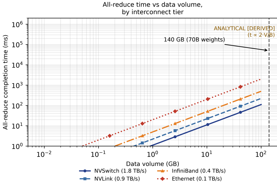
FIGURE 9.1: All-reduce time vs data volume, by interconnect tier (ANALYTICAL [DERIVED] model). The plot is marked in-figure as analytical, not measured network performance: completion time scales as 2 \cdot V/B (roughly twice the data across the tree), and the four tiers differ by effective bandwidth. The 140 GB vertical line marks the 70B FP16 weight footprint. [DERIVED: t = 2 \cdot V/B ; bandwidths are vendor nominal, not benchmarked]
