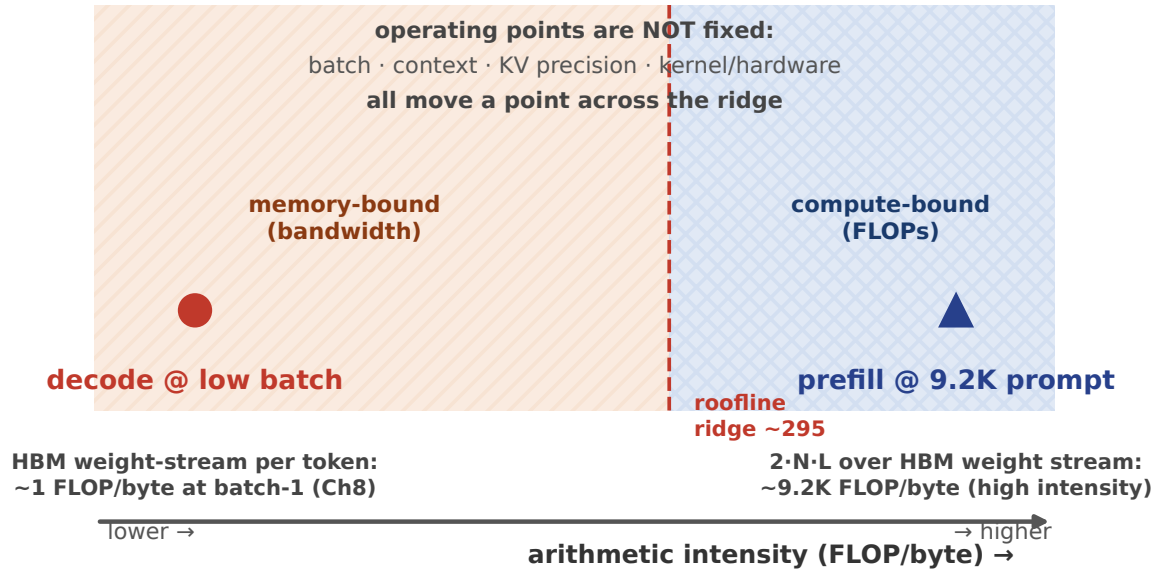
FIGURE 2.2: Prefill and decode sit on an arithmetic-intensity continuum, split by the roofline ridge. Low-batch decode (streaming weights per token) lands at ~1 FLOP/byte — the memory-bound side; long-prompt prefill lands at high intensity — the compute-bound side. These are operating points, not fixed identities: batch, context, precision, kernel and hardware all move a point across the ridge. [ILLUSTRATIVE conceptual, roofline developed in Ch 8]
