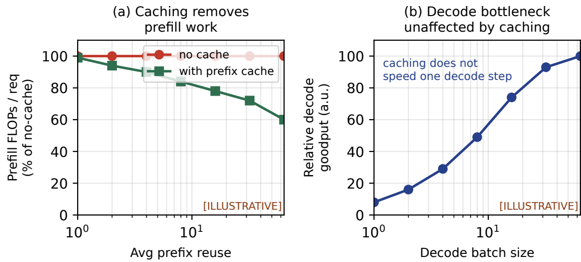
FIGURE 15.2: Prefix caching and batching affect different serving phases: caching reduces prefill work; batching raises decode goodput
