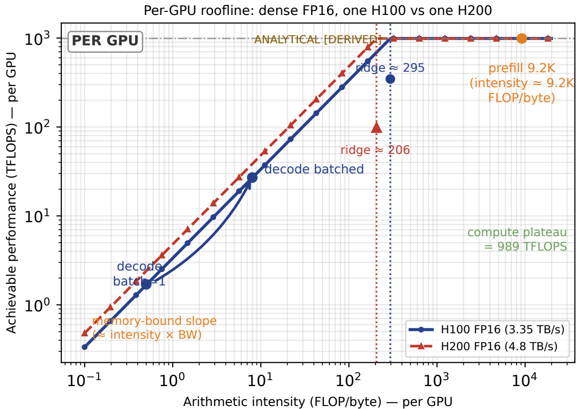
FIGURE 8.2: Per-GPU roofline for dense FP16, one H100 vs one H200 (a per-GPU chart, not a host-level one). Compute ceiling and HBM bandwidth are single-GPU quantities here (989 TFLOPS, 3.35 / 4.8 TB/s), so the ridge point and the memory-bound slope are per-GPU. Prefill (9.2K input) sits to the right of the ridge, on the compute-bound plateau; decode (batch=1) sits to the left, on the memory-bound slope, and continuous batching climbs the slope as batch grows. The ridge classification (compute- vs memory-bound) is unchanged by ideal N-way replication because both peak FLOP/s and HBM bandwidth scale with GPU count; host-level attainable performance additionally depends on sharding and communication. [DERIVED from 1P: vendor datasheet]
