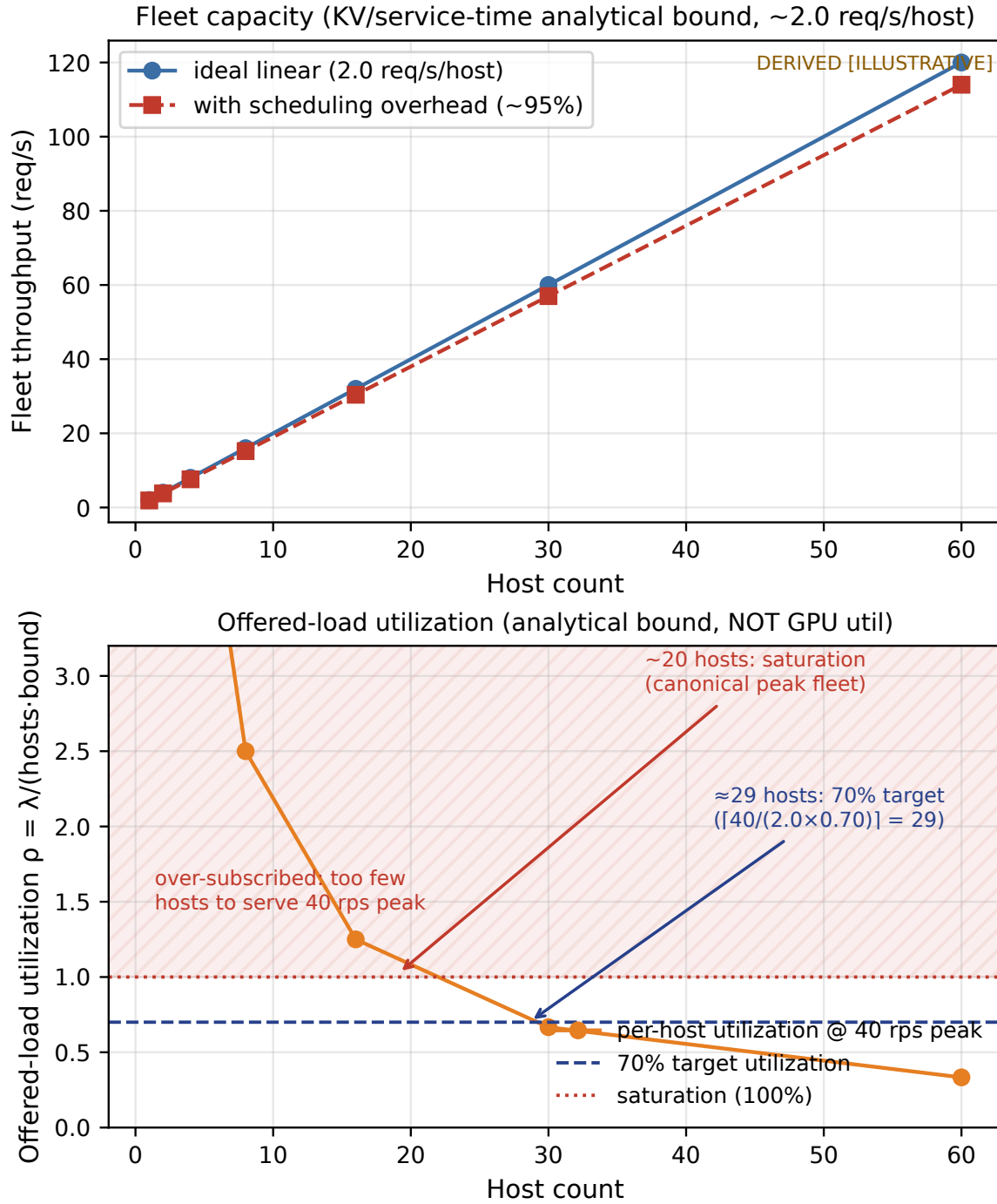
FIGURE 20.1: Fleet capacity (KV/service-time analytical bound, ~2.0 req/s/host) and per-host offered-load utilization, vs. host count at the canonical peak load (40 rps). Top panel: capacity against host count from the KV/service-time analytical bound (~2.0 req/s/host), with a ~95% scheduling-overhead line. Bottom panel: per-host offered-load utilization ( \rho = \lambda / (\text{hosts} \cdot \text{bound}) ) at the canonical 40 rps peak — this is an analytical-capacity utilization, NOT GPU utilization. This is the honest quantity for the tail: p99 is driven by per-host utilization, not by host count alone. Adding hosts lowers per-host utilization (more headroom) hence lowers the expected tail; the 70%-utilization and 100%-saturation reference lines show the provisioning target. The tail also depends on the arrival process, scheduling policy, batching, and the service-time distribution, which a provisioning model alone does not capture. The ~2.0 req/s line is the KV/service-time analytical bound, not a benchmarked serving throughput. [ILLUSTRATIVE][DERIVED]
