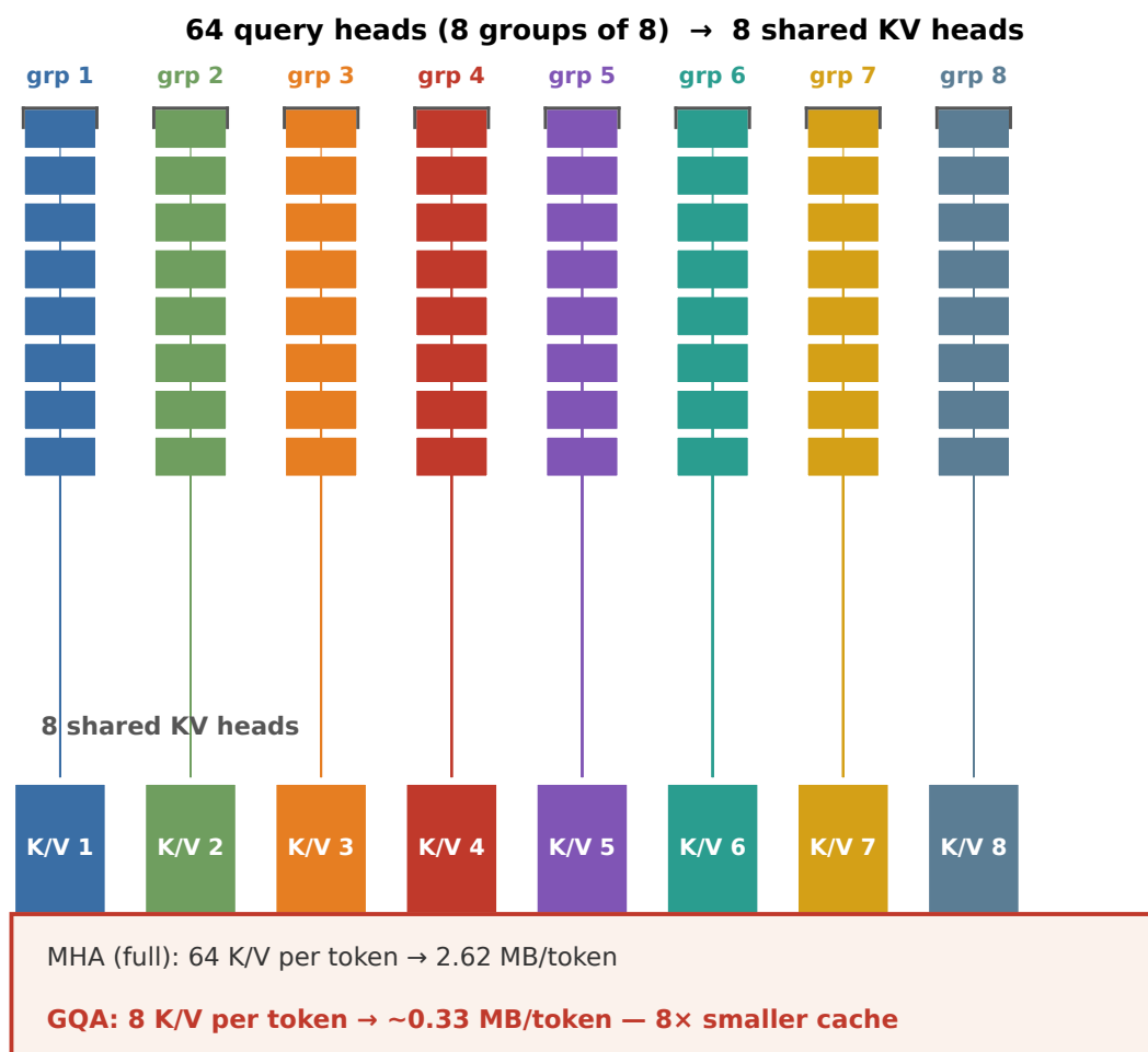
FIGURE 7.1: Grouped-Query Attention cuts per-token KV
