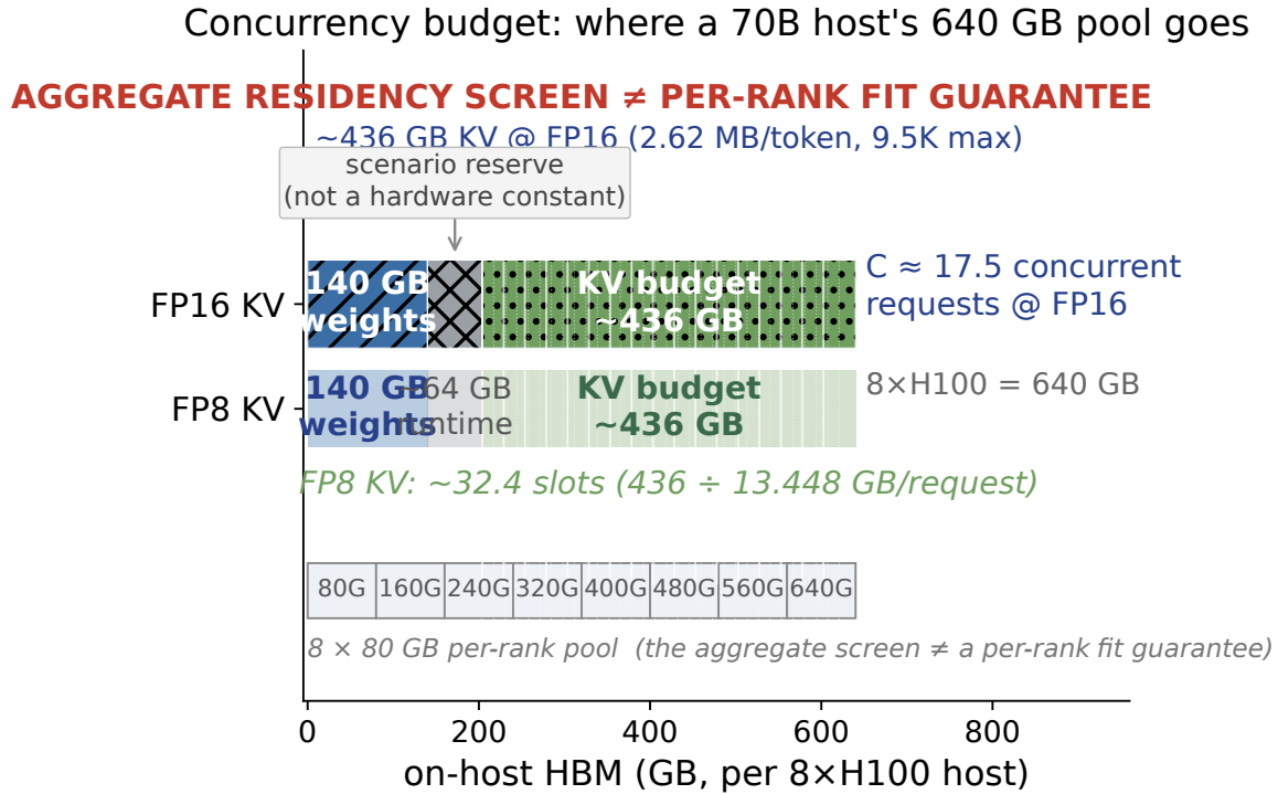
FIGURE 7.4: The concurrency budget: where a 70B host's 640 GB pool goes. Aggregate-feasibility caveat: the 640 GB figure is an aggregate across eight 80-GB H100s, not a single freely-allotable heap. Whether a given allocation actually fits depends on tensor-parallel sharding, KV partitioning, replication, runtime layout, per-rank fragmentation, workspace requirements, and communication topology — so “total bytes < total HBM” is a necessary but not sufficient test. Per-rank fit and sharding must also be validated (Chapters 9–10). [ILLUSTRATIVE][DERIVED]
