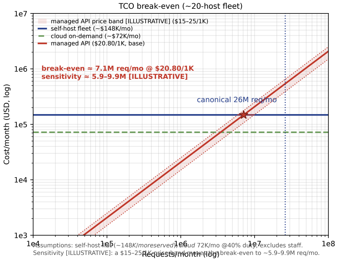
FIGURE 16.1: TCO break-even: self-hosted vs managed API [ILLUSTRATIVE][DERIVED]
