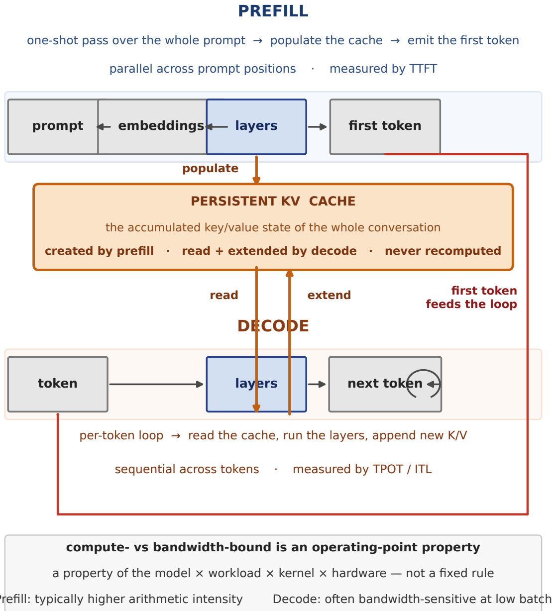
FIGURE 2.1: The canonical end-to-end inference pipeline: prompt to generated tokens, divided into PREFILL (top) and DECODE (bottom). Prefill is the one-shot parallel burst that populates the KV cache and yields the first token — it commonly occupies a higher-arithmetic-intensity regime, straining compute, and is measured by TTFT. Decode is the sequential autoregressive loop that reuses the cached K/V and re-reads weights every step — it commonly occupies a lower-arithmetic-intensity regime, straining HBM bandwidth and capacity, and is measured by TPOT/ITL. These are useful heuristics, not universal laws: which phase is actually compute- or bandwidth-bound is a property of the model × workload × kernel × hardware operating point (developed through the roofline framework in Ch 8). [ILLUSTRATIVE conceptual]
