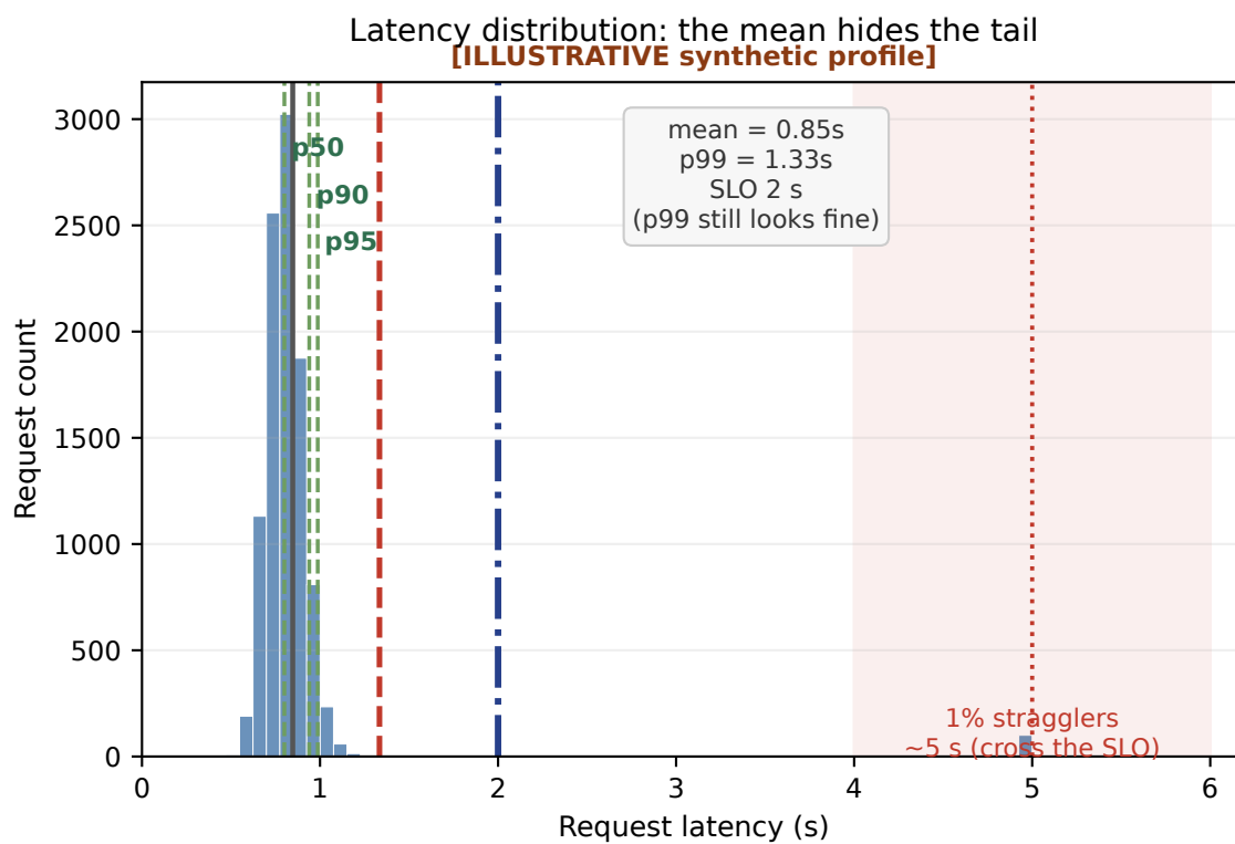
FIGURE 6.2: Request-latency distribution: p50/p90/p95/p99 and the mean
