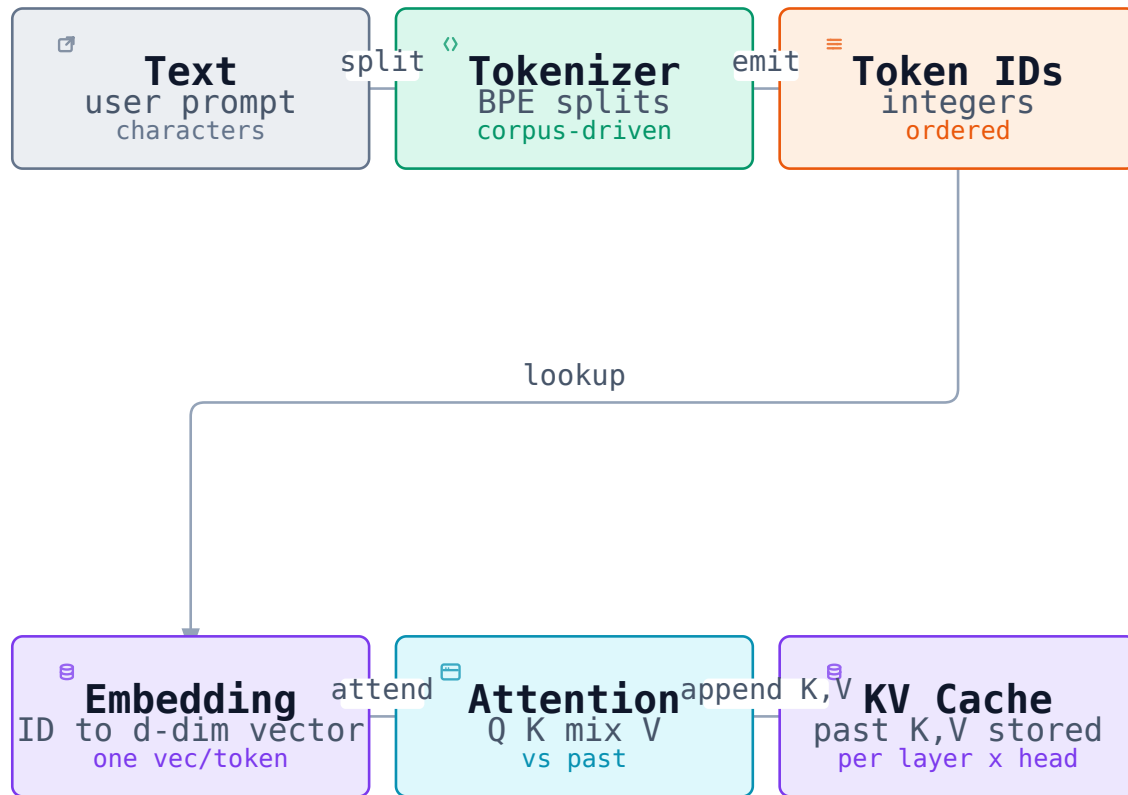
FIGURE 1.2: How a token travels: text → tokenizer → IDs → embedding → attention → KV cache [ILLUSTRATIVE conceptual]
