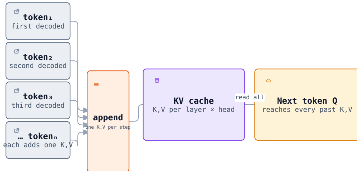
FIGURE 1.1: The KV cache: every decoded token adds one K+V per layer per head [ILLUSTRATIVE conceptual]
