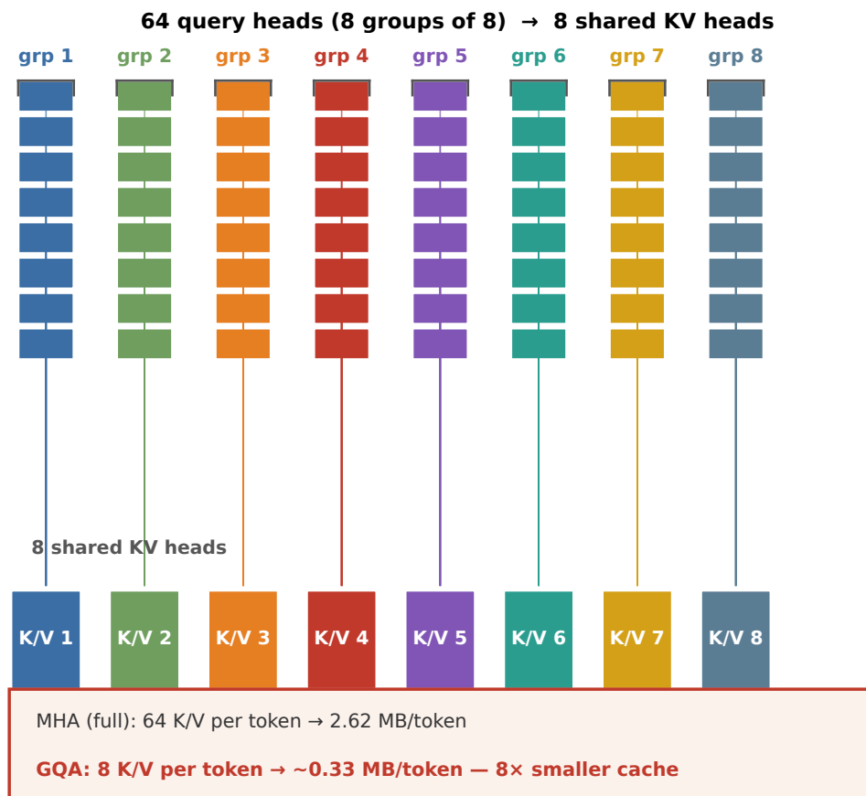
FIGURE 7.1: Grouped-Query Attention cuts per-token KV
