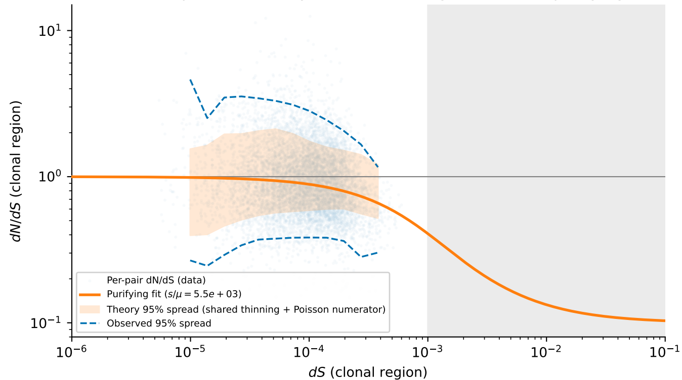
Observed spread vs theory (shared thinning) around the purifying fit
