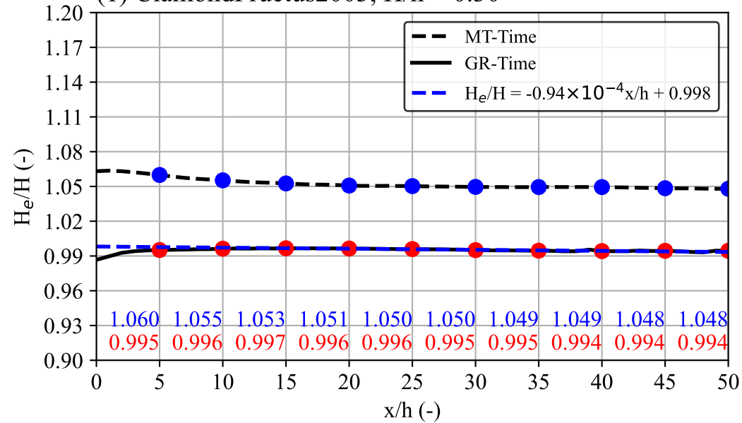
(3) ClamondFructus2003, H/h = 0.50
