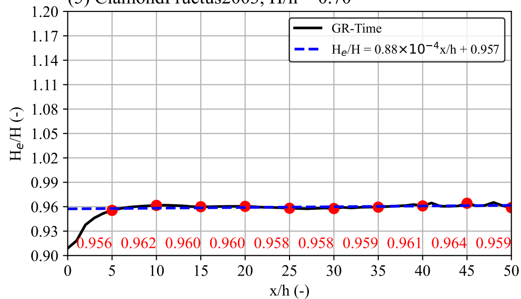
(5) ClamondFructus2003, H/h = 0.70
