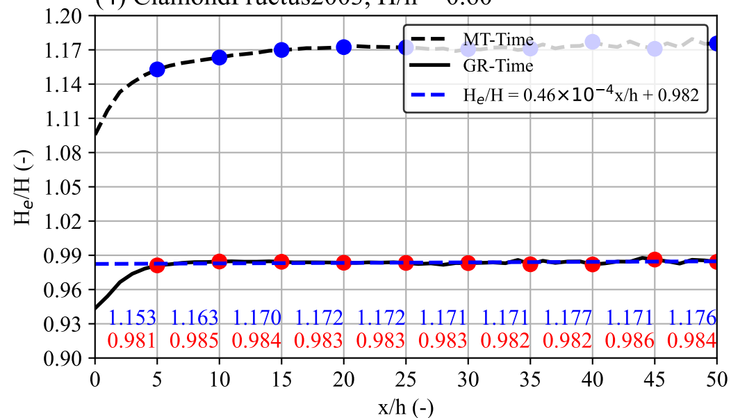
(6) ClamondFructus2003
