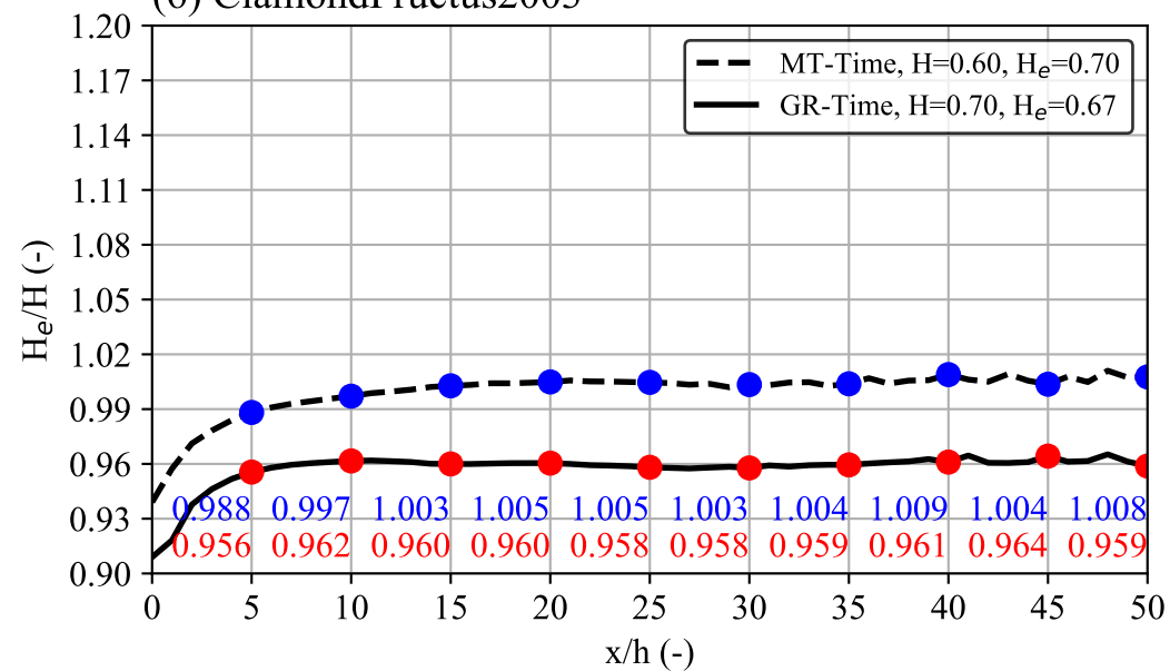
(6) ClamondFructus2003
