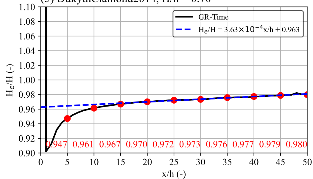
(5) DukythClamond2014, H/h = 0.70
