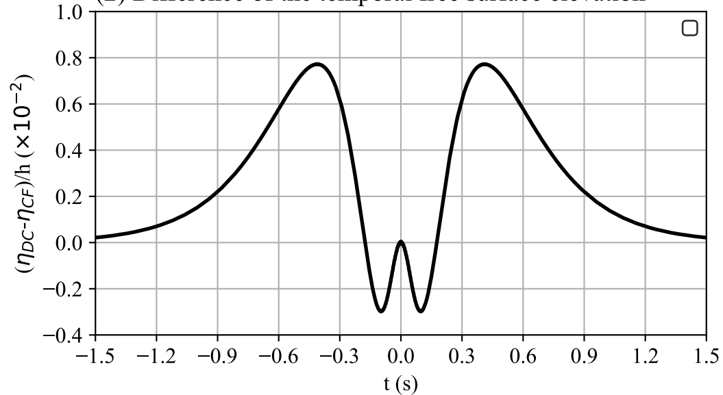
(2) Difference of the temporal free surface elevation
