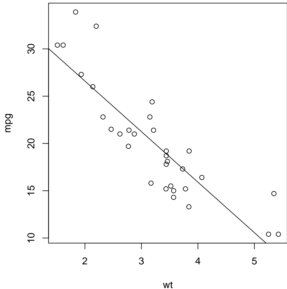
Regression of MPG on Weight
