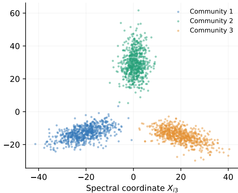
True communities
