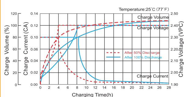
Charge Characteristic Curve for Cycle Use(IU)
