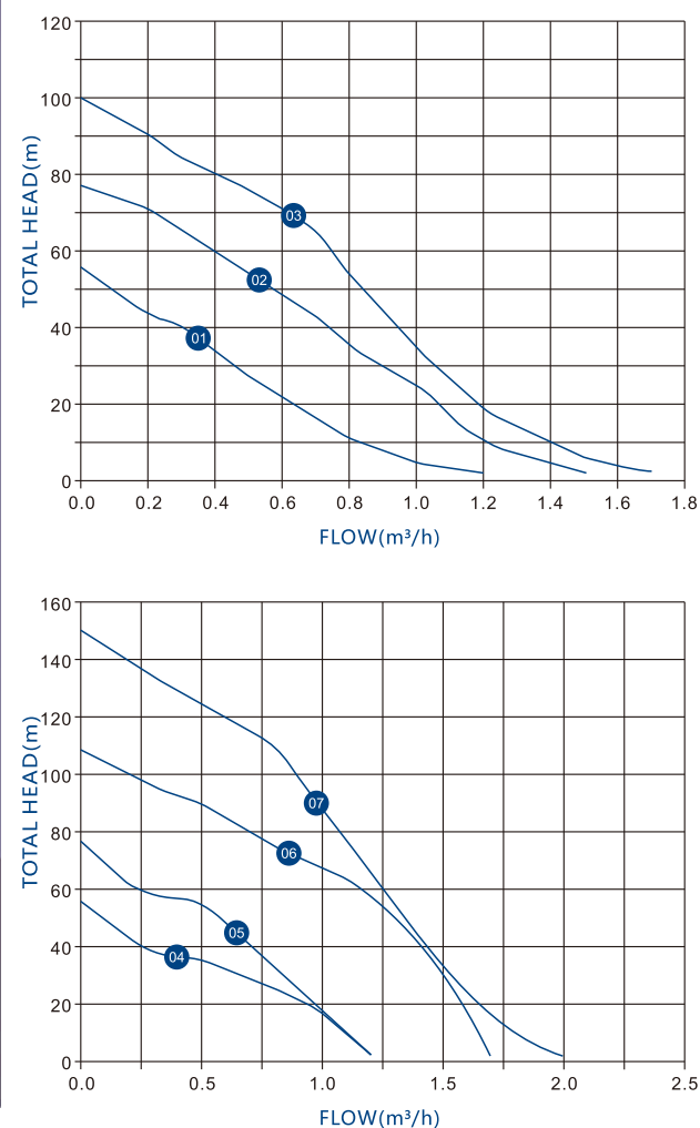
PERFORMANCE CURVES
