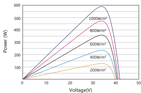
P-V CURVES OF PV MODULE(595W)
