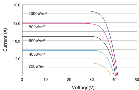
I-V CURVES OF PV MODULE(595 W)
