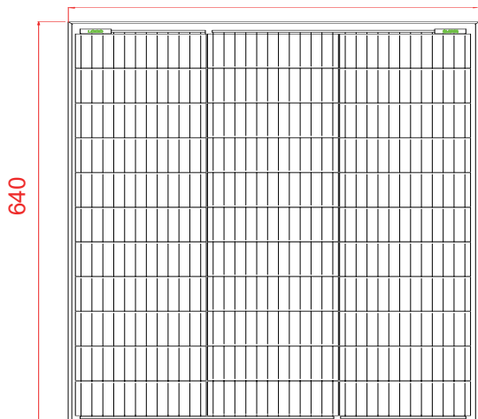
Dimension of PV Modules Unit: mm
