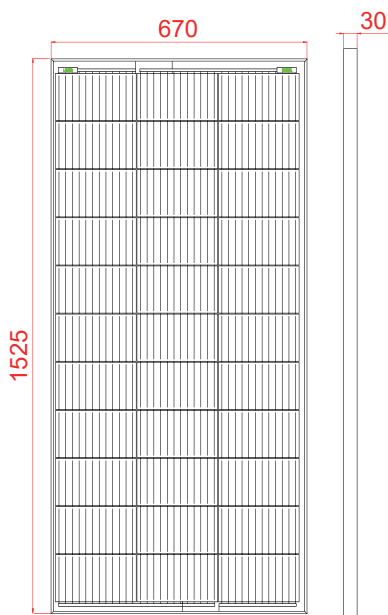
Dimension of PV Modules Unit: mm
