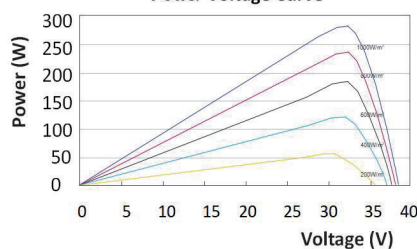
Power-Voltage Curve
