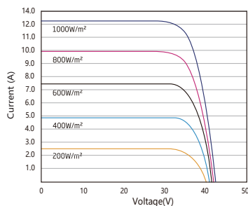
I-V CURVES OF PV MODULE
