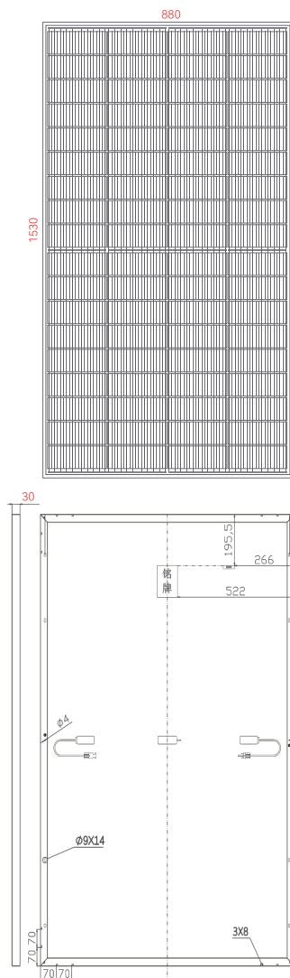
Dimension of PV Modules Unit: mm
