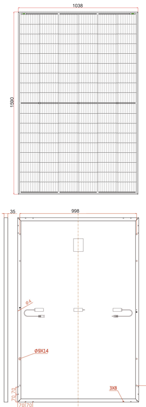
Dimension of PV Modules Unit: mm
