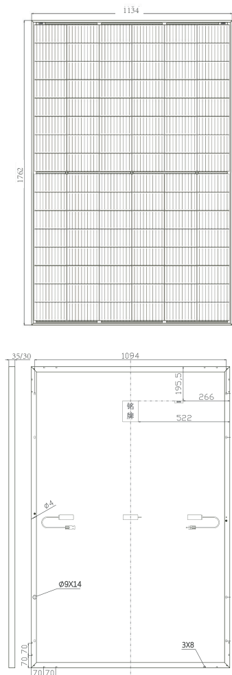
Dimension of PV Modules Unit: mm
