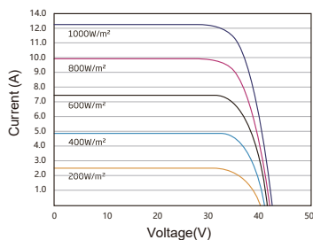
I-V CURVES OF PV MODULE(460W)
