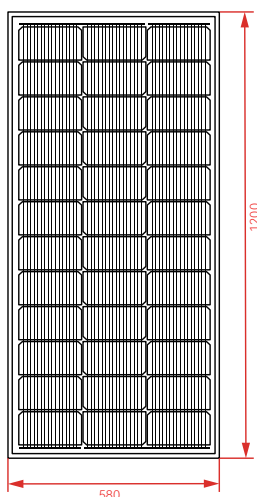
Dimension of PV Modules Unit: mm
