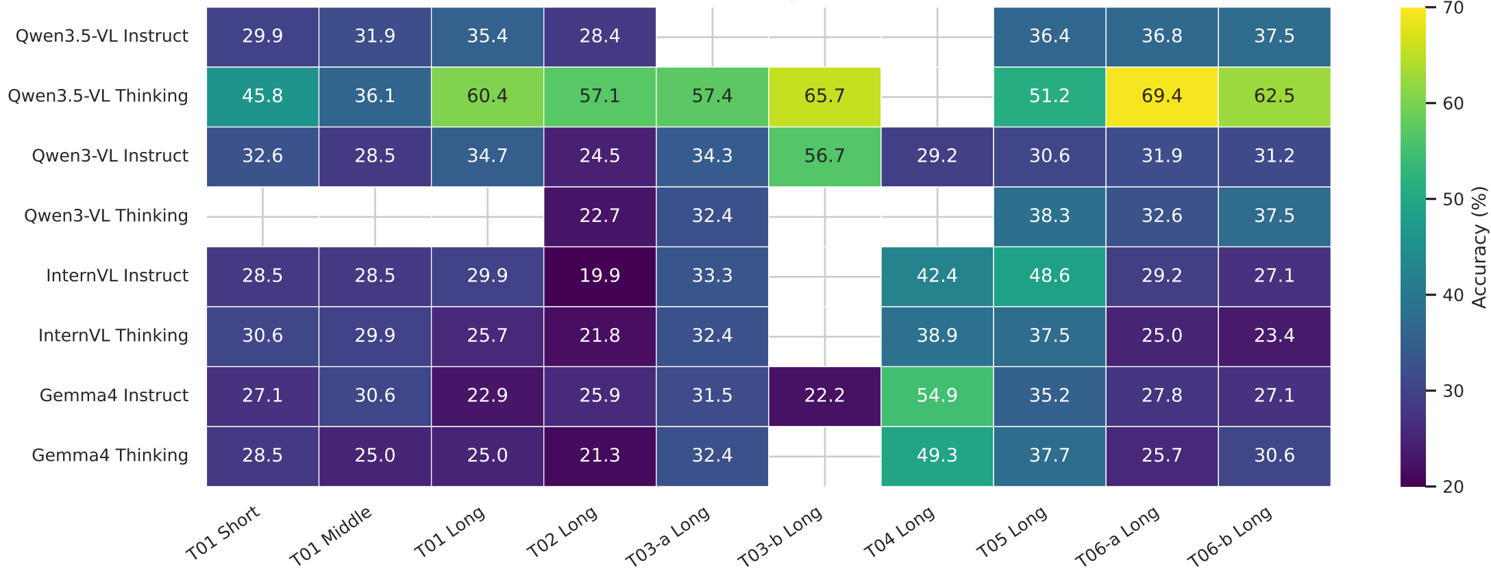
COMFORT accuracy across tests
