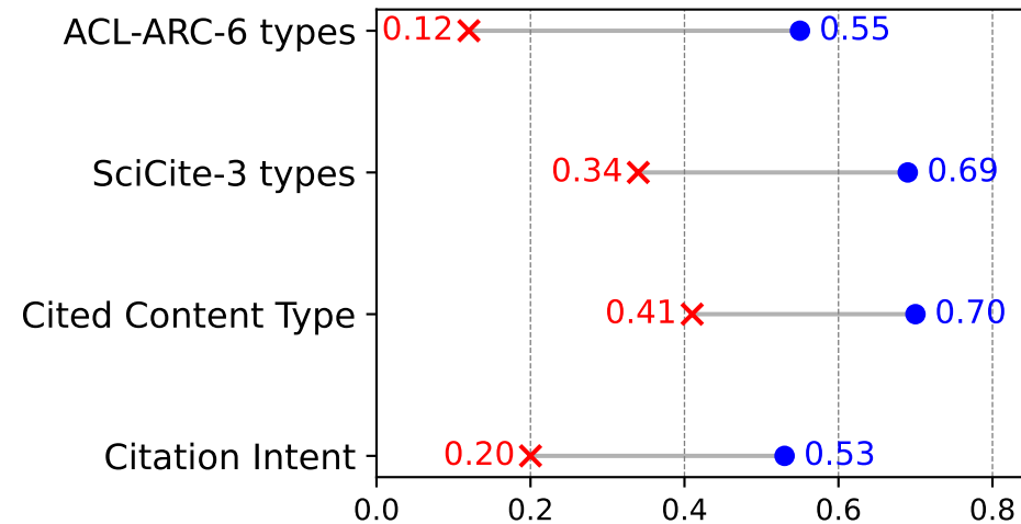
Fine-tuned SciBERT
