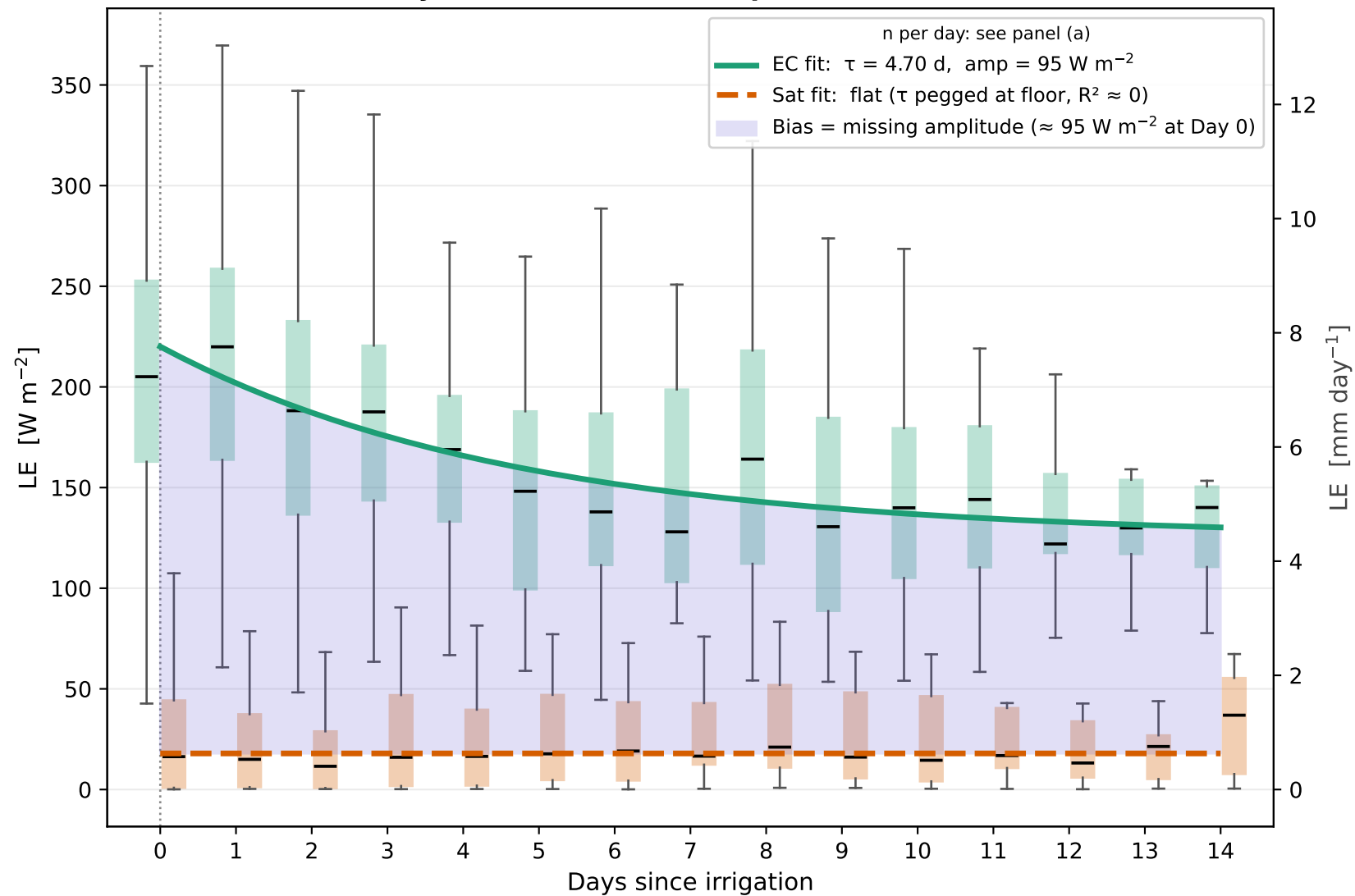
(b) EC vs Sat recovery — same events, two products
