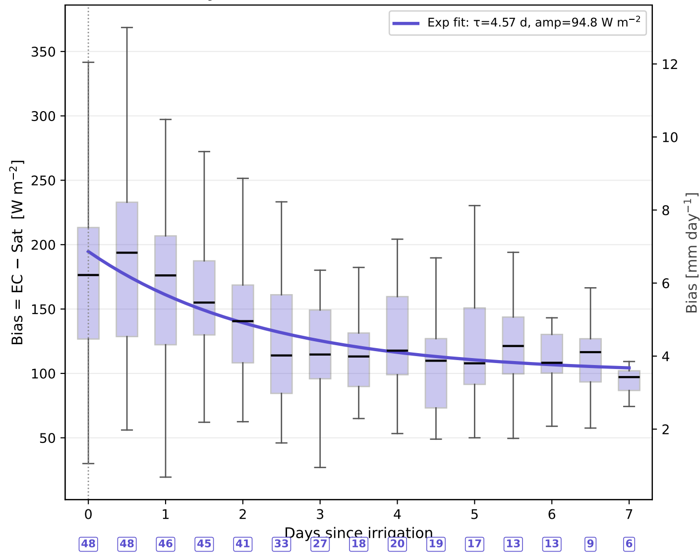
(a) Bias recovery (n events = 48, R^2 = 0.86 )
