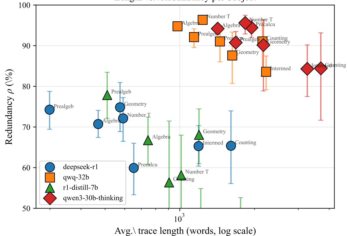
Length vs. Redundancy per Subject
