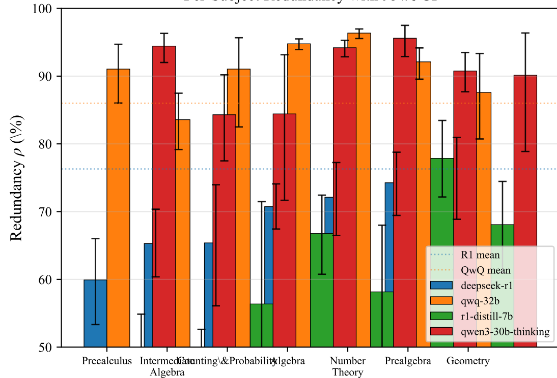
Per-Subject Redundancy with 95% CI
