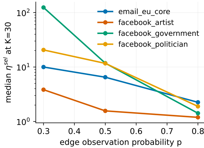
Figure 3: Median \eta^{\text{sel}} at K = 30 against the edge observation probability p , one line per network (log scale). The error rises as the graph is observed less, on all 4 networks; over the same range the realized ratio falls only from no worse than 0.988 to between 0.882 and 0.963, while the certified bound L_{30}(\eta^{\text{sel}}) falls by up to a factor 64.
