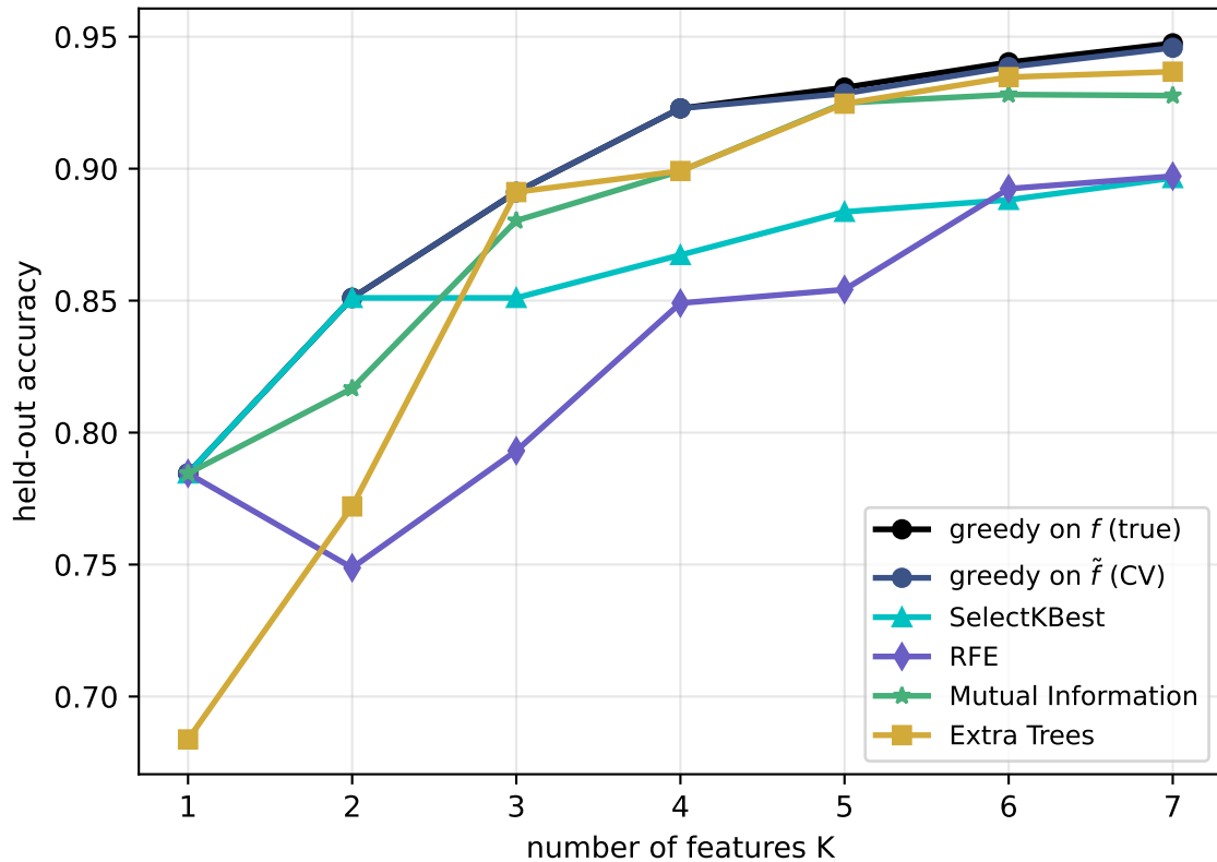
airline (median over 10 seeds)
