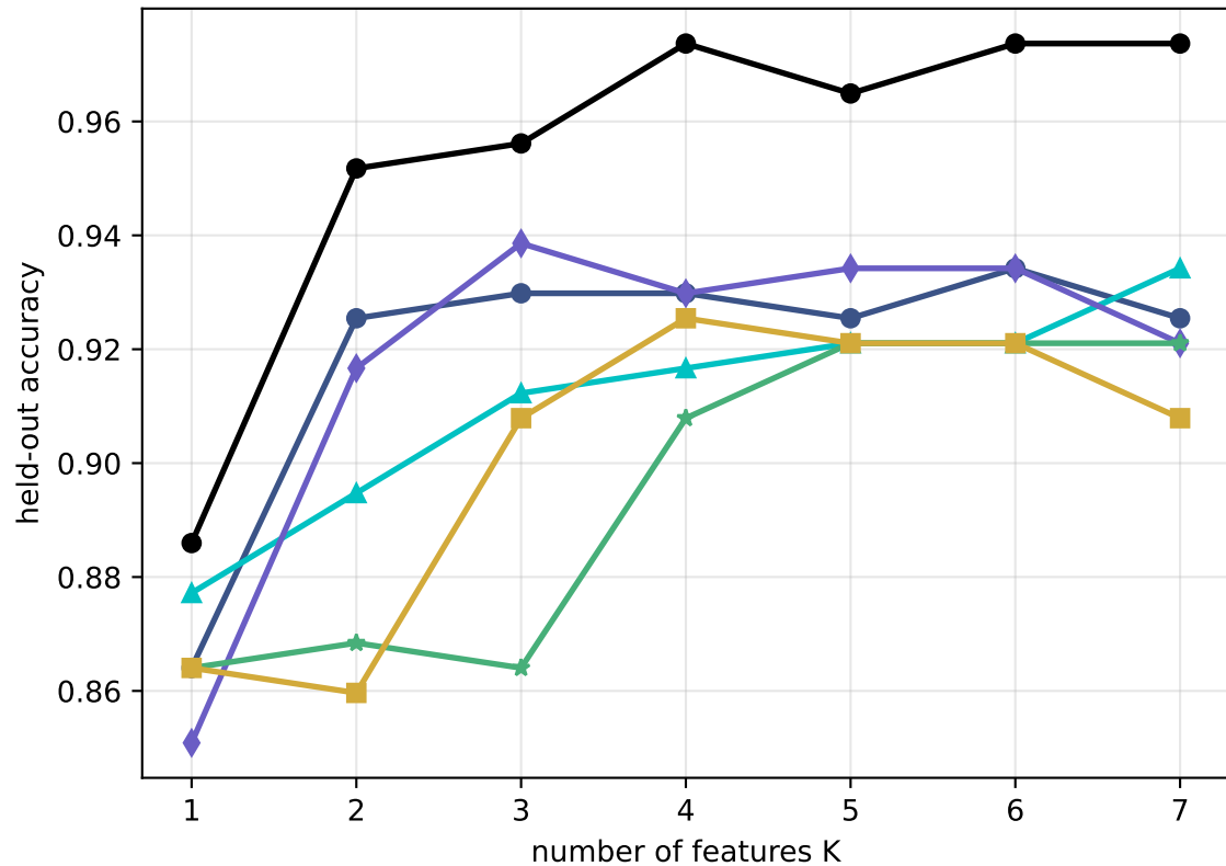
breast_cancer (median over 10 seeds)
