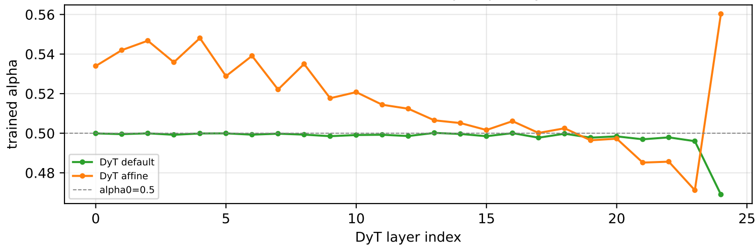
Classification: trained alpha per layer
