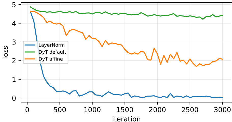
Classification training loss
