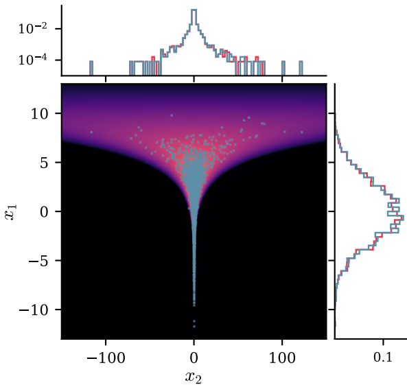
t-EDM ( \nu = 4, 20 ) + CVaR-GPA
