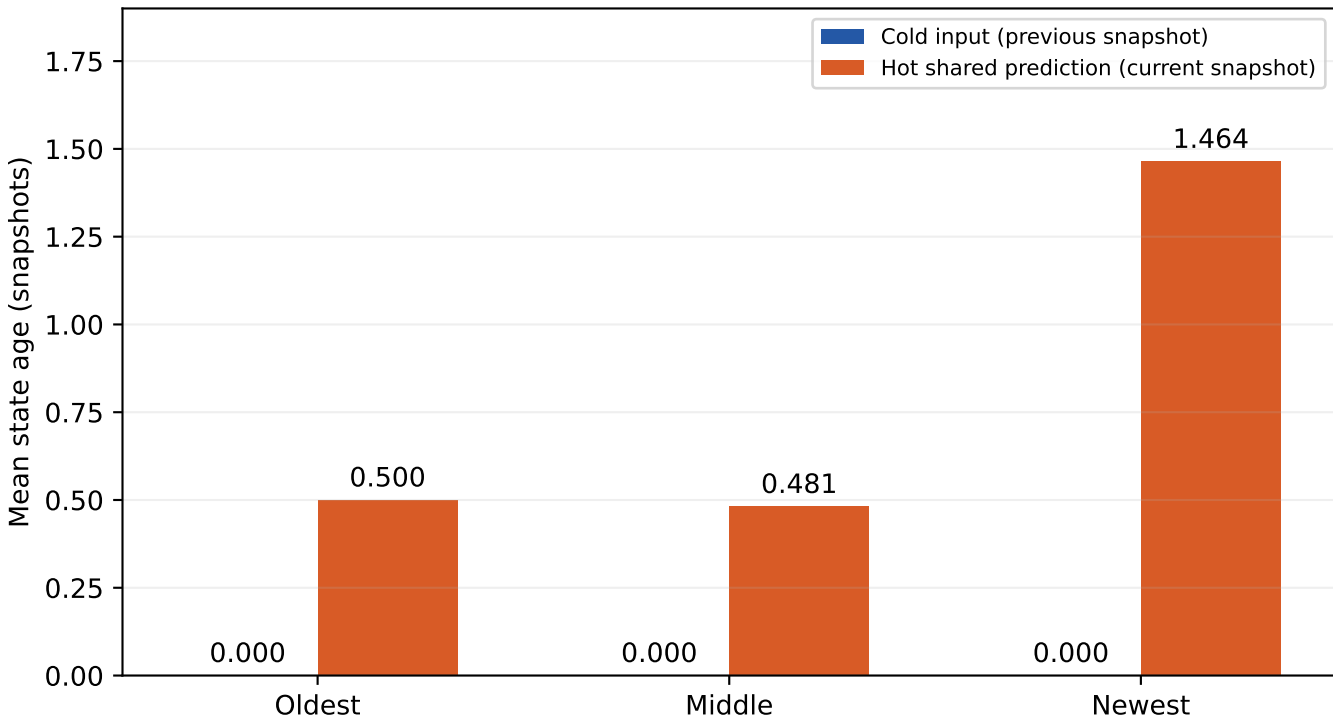
Flickr | GConvGRU | W=3 | first training epoch
