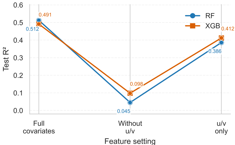
(a) Absolute predictive skill
