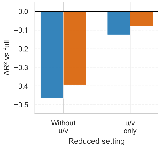
(b) Skill loss after feature removal
