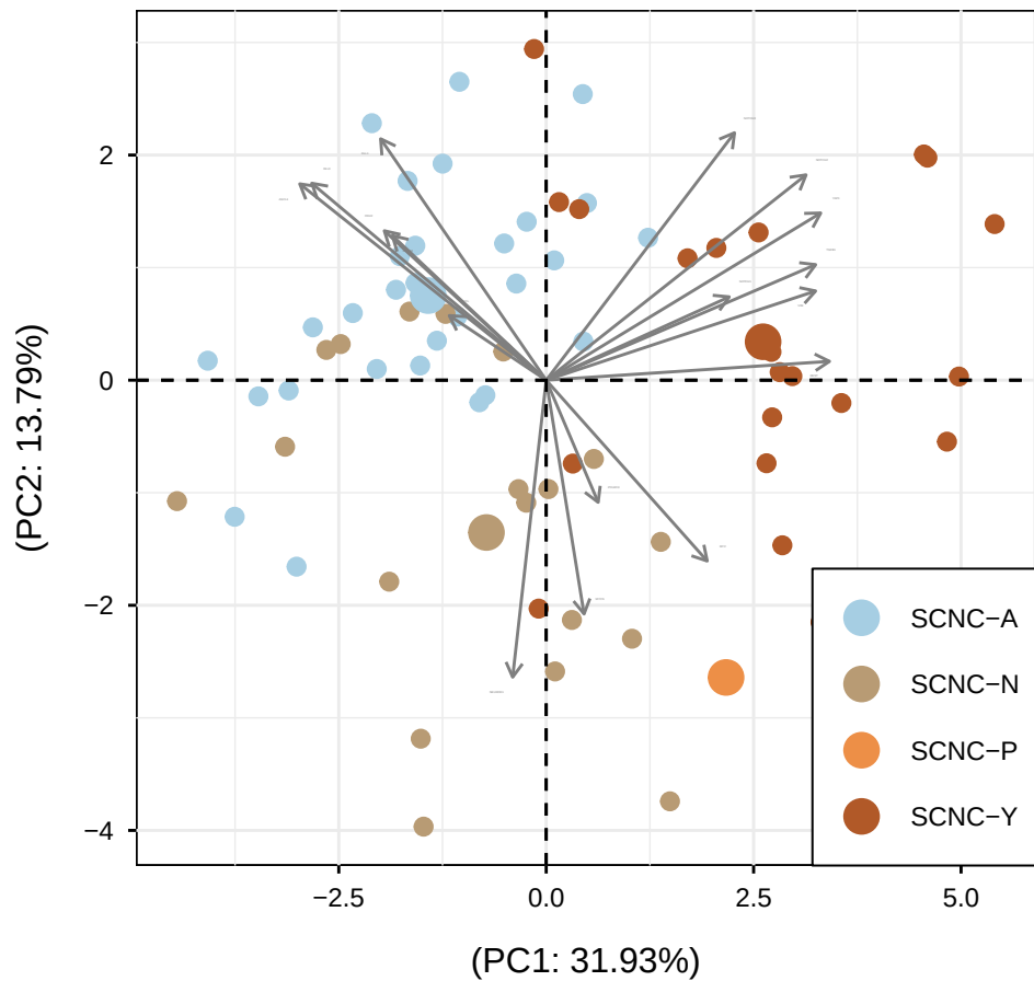
PCA-Biplot
