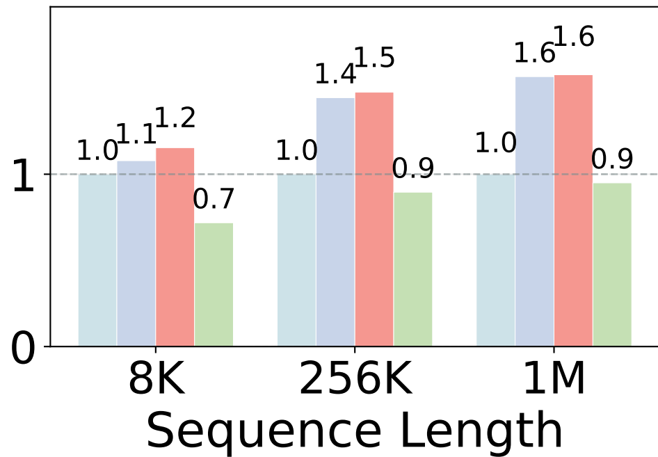
Latency Speedup
