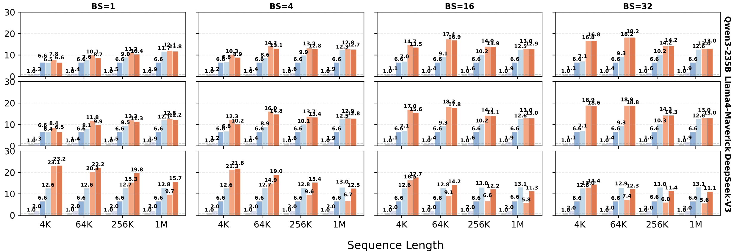
Latency Speedup
